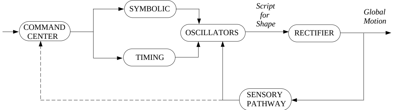
Figure 4. Architecture for Motion Control
