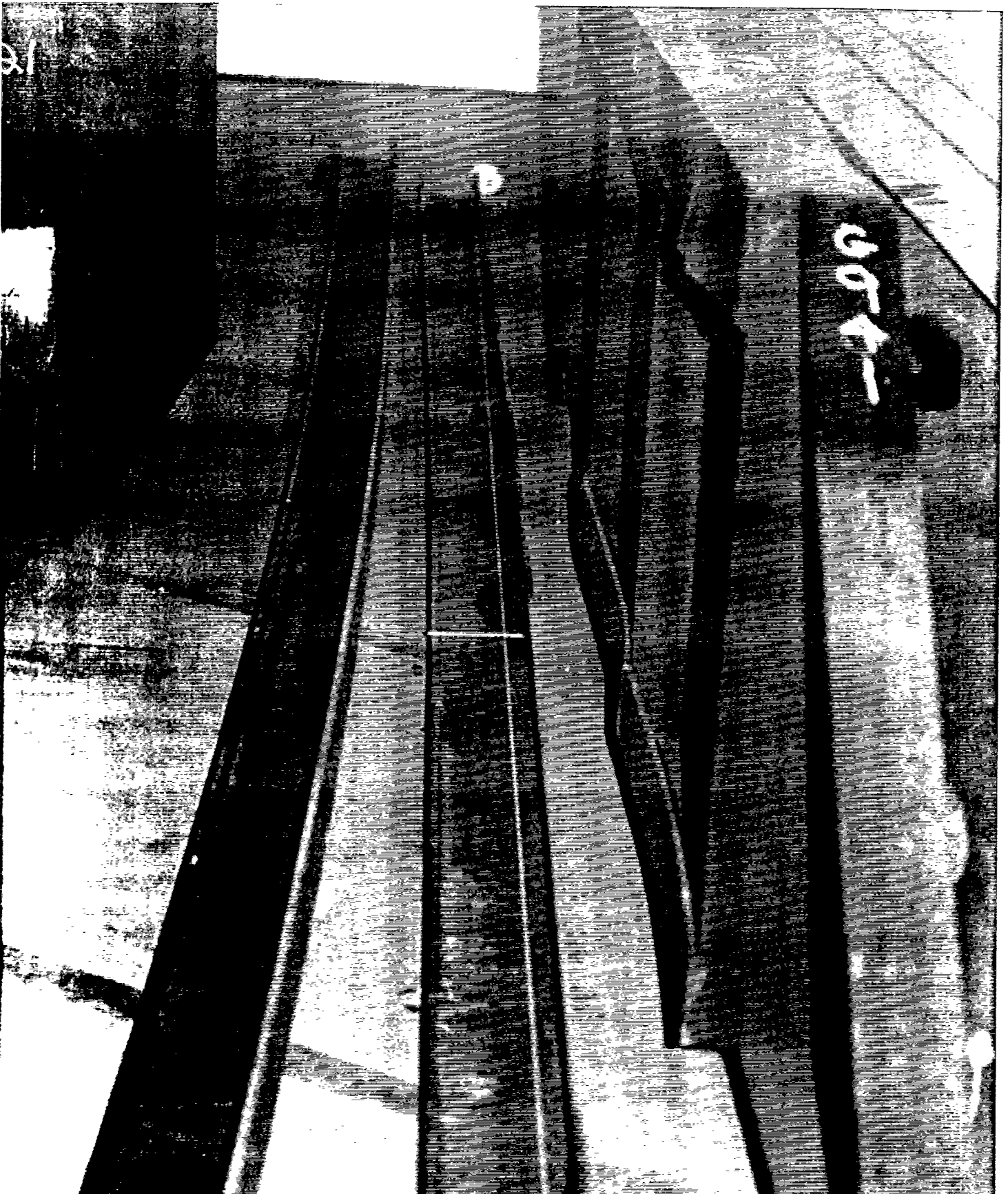
22. Distortion of dual-torch plasma cut W6X20 beam beams, dry (left) vs. wet
