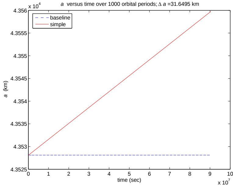
Figure 4.12: Simple Controller Case Behavior of a for Nominal Reflection Coefficients, 1000 Orbits and an Area Factor of 1, Overlaid with the Corresponding Baseline Case Behavior of a .
