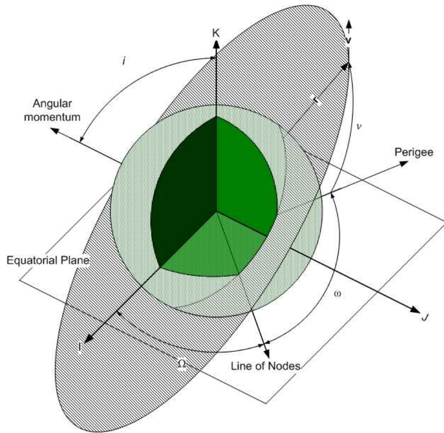
Figure 3.1: COE Geometry. The COE a and e are difficult to depict in this figure, and thus are omitted.
