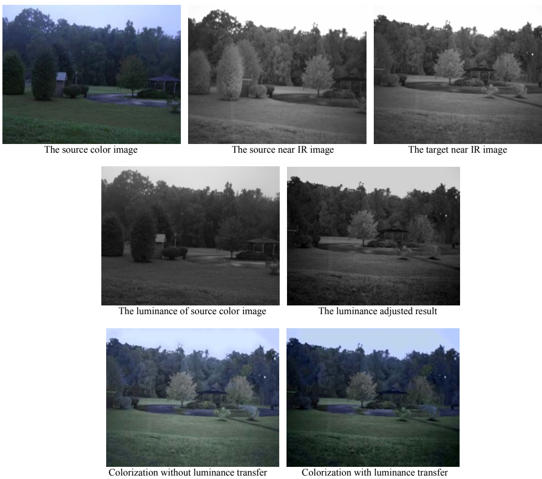
Figure 54: The second example of luminance and color transfer.
