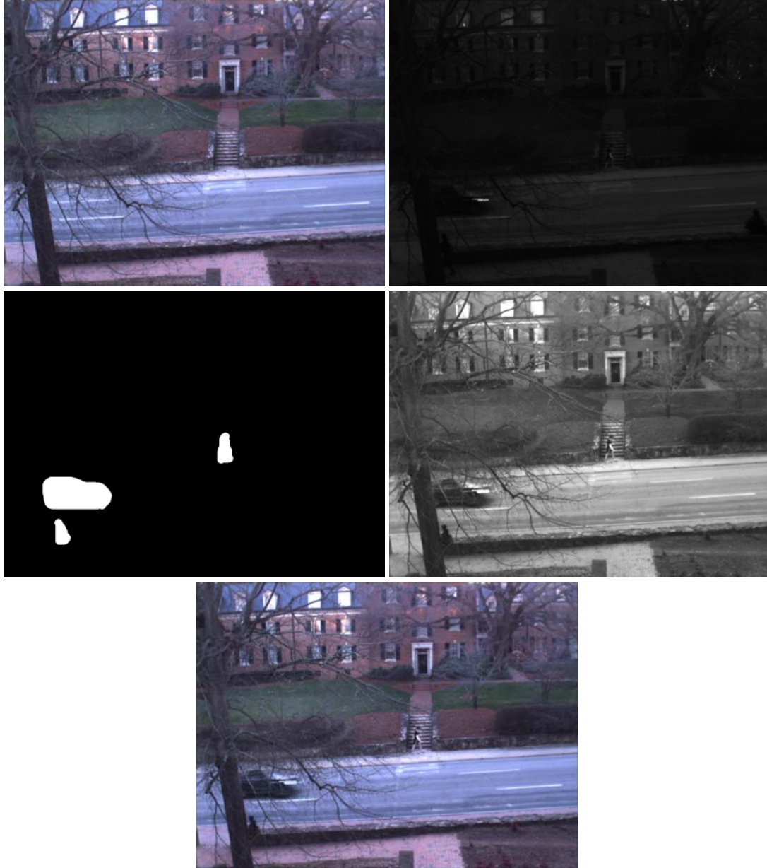
Figure 16: Illustration of mixing gradient fields from daytime and nighttime images. Upper Left: a daytime RGB image; Upper Right: a grayscale nighttime image; Middle Left: a mask displaying areas of difference between the two images; Middle Right: Poisson interpolation of the mixed gradient fields as defined by the mask; Bottom Center: Poisson interpolated image with chrominance copied from daytime RGB image.
