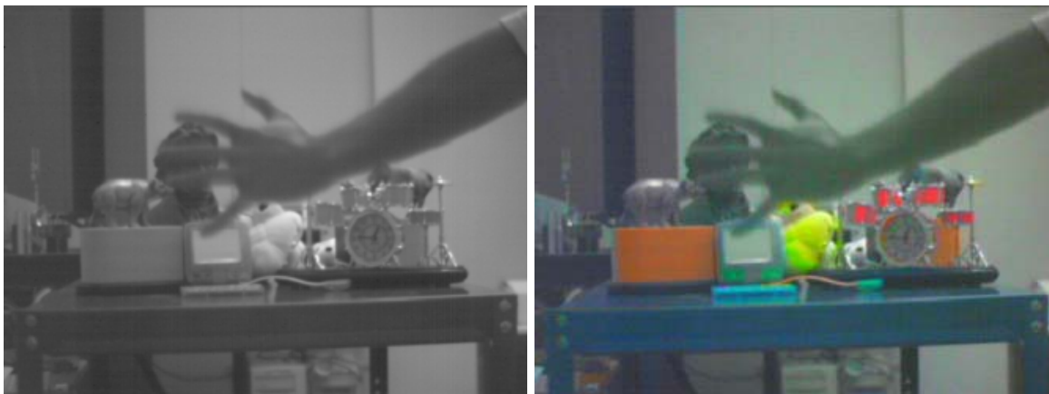
Figure 37: Results from a failed chrominance transfer. Left: SWIR image interpolated with the RGB boundary conditions. Right: Chrominance transfer from the RGB image to the interpolated image.
