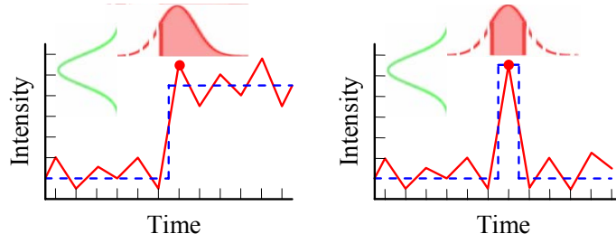
Figure 5: Left: The bilateral filter recovers the signal (blue) from the noisy input (red). Right: The bilateral filter is unable to attenuate the shot noise because no other pixels fall within the intensity dissimilarity Gaussian.
