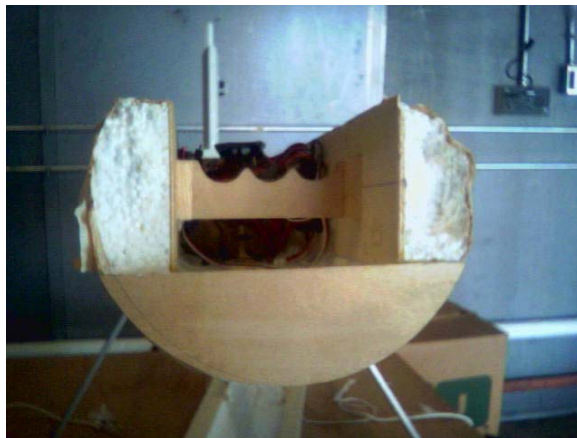
Figure 6. Fuselage Cross Section Prior to Completed Repairs.
