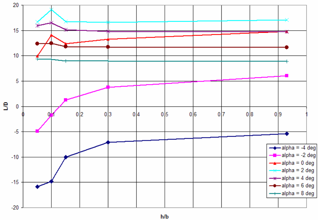
Figure 72: Lambda UCAV L/D vs. (h/b) 80 mph
