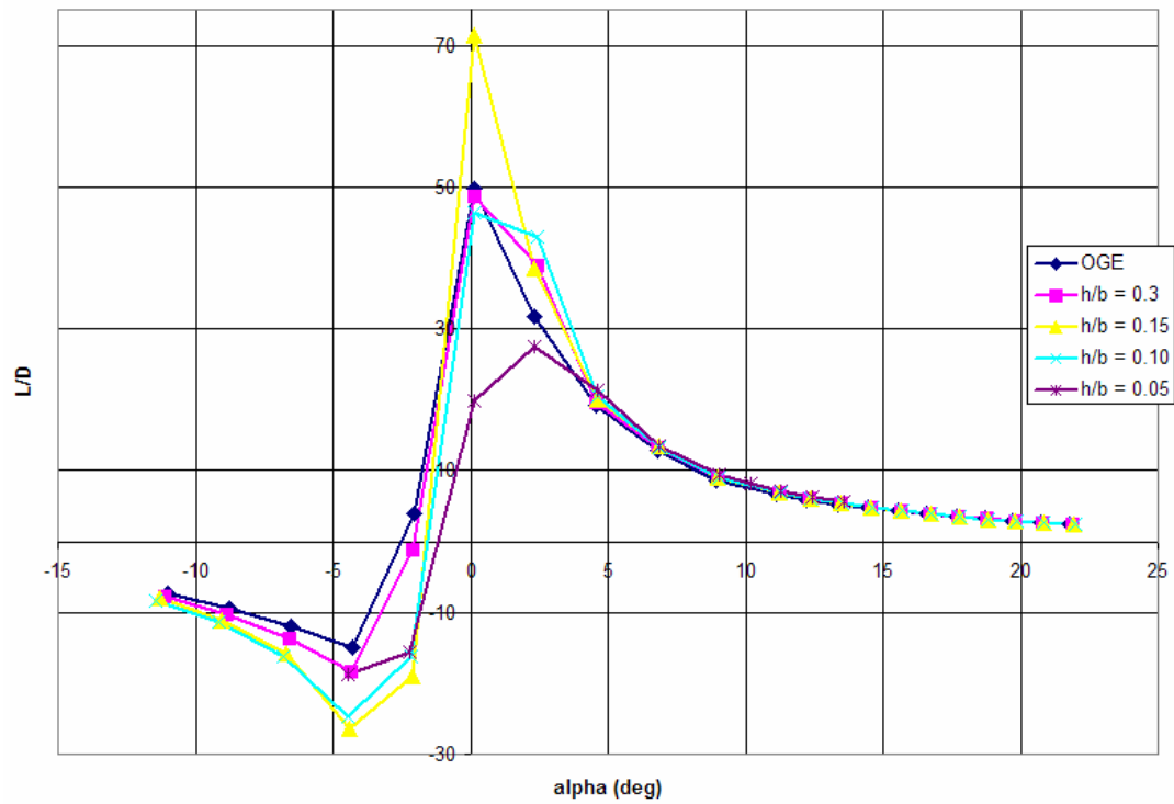
Figure 52: Lambda UCAV Ground Effect - L/D vs. alpha, 40 mph
