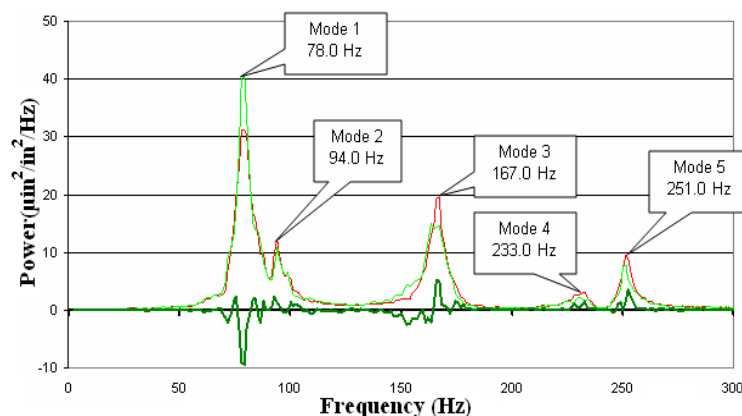
Figure 5.29: Natural Modes via Strain Gage - 20,000 feet, 0.6 Mach [14]
