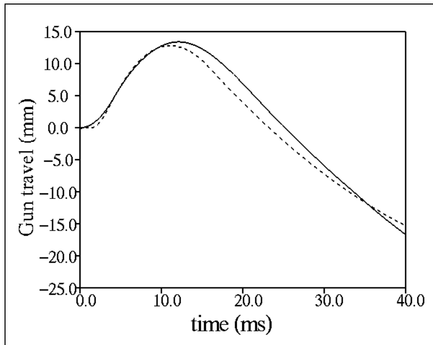
Figure 12. Gun travel; light piston, early vent, low-pressure group: shot 2-6-3 (line) and simulation (dot).
