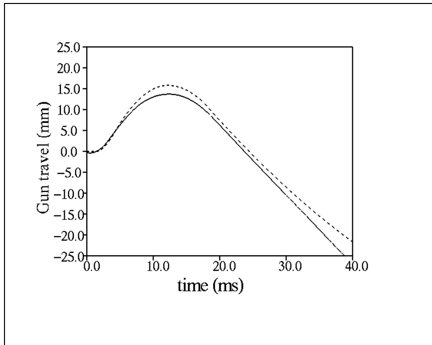
Figure 18. Gun travel; heavy piston, early vent, low-pressure group: shot 2-3-4 (line) and simulation (dot).
