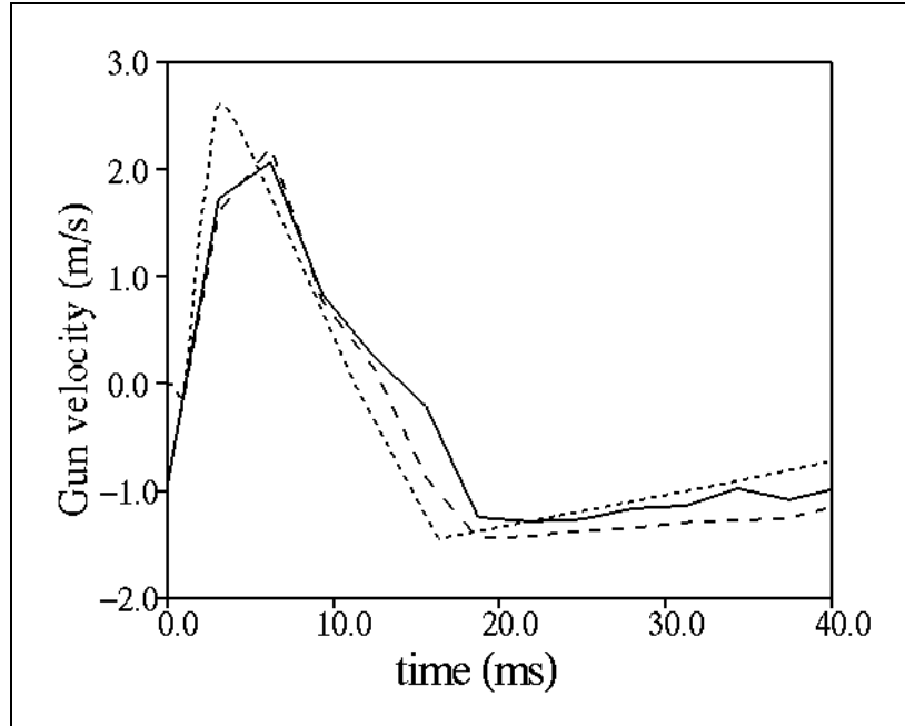
Figure 13. Gun velocity; light piston, early vent, high-pressure group: shot 2-6-1 (line), shot 2-6-2 (dash), and simulation (dot).
