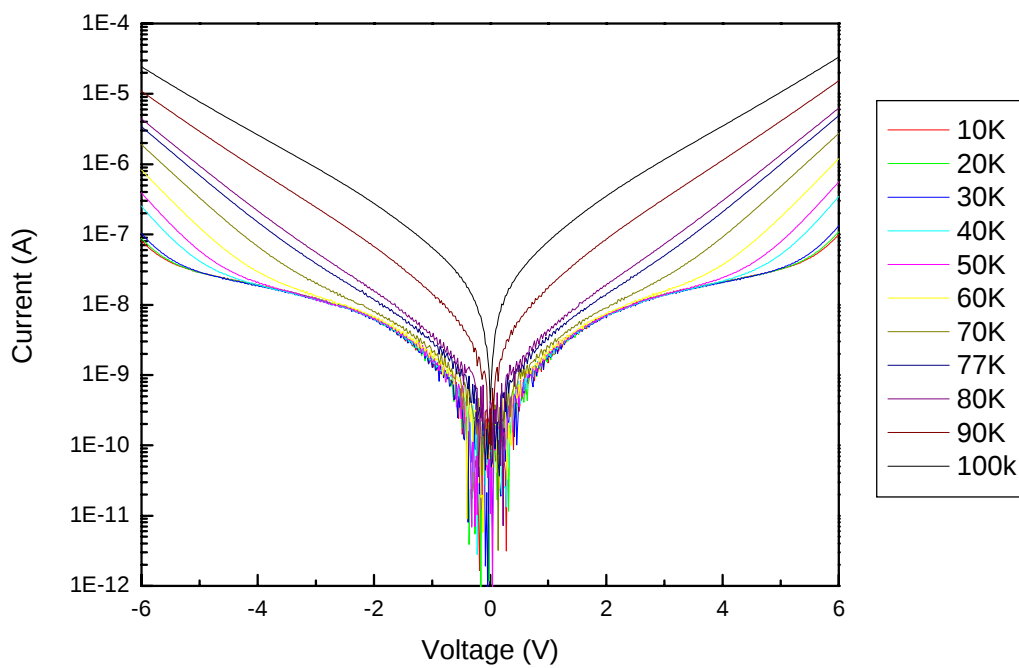
Figure 19. MWIR detector I-V curves without the aluminum shield in place.
