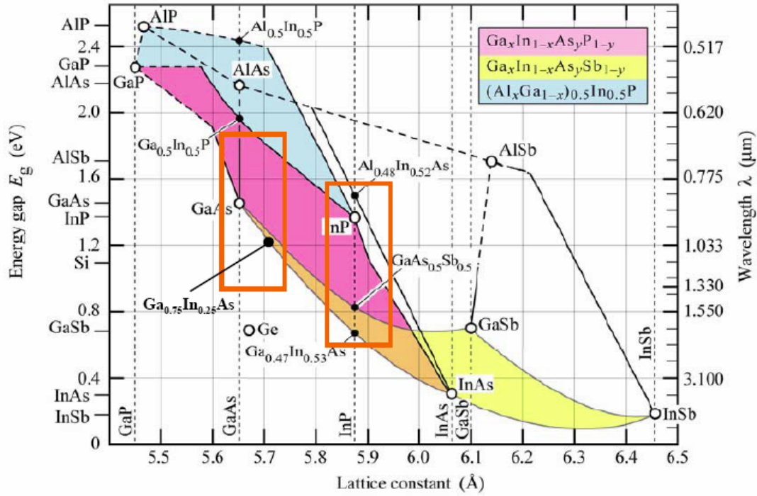
Figure 15. Plot of energy bandgap vs. lattice constants for major III-V compounds (After Ref. [14]).
