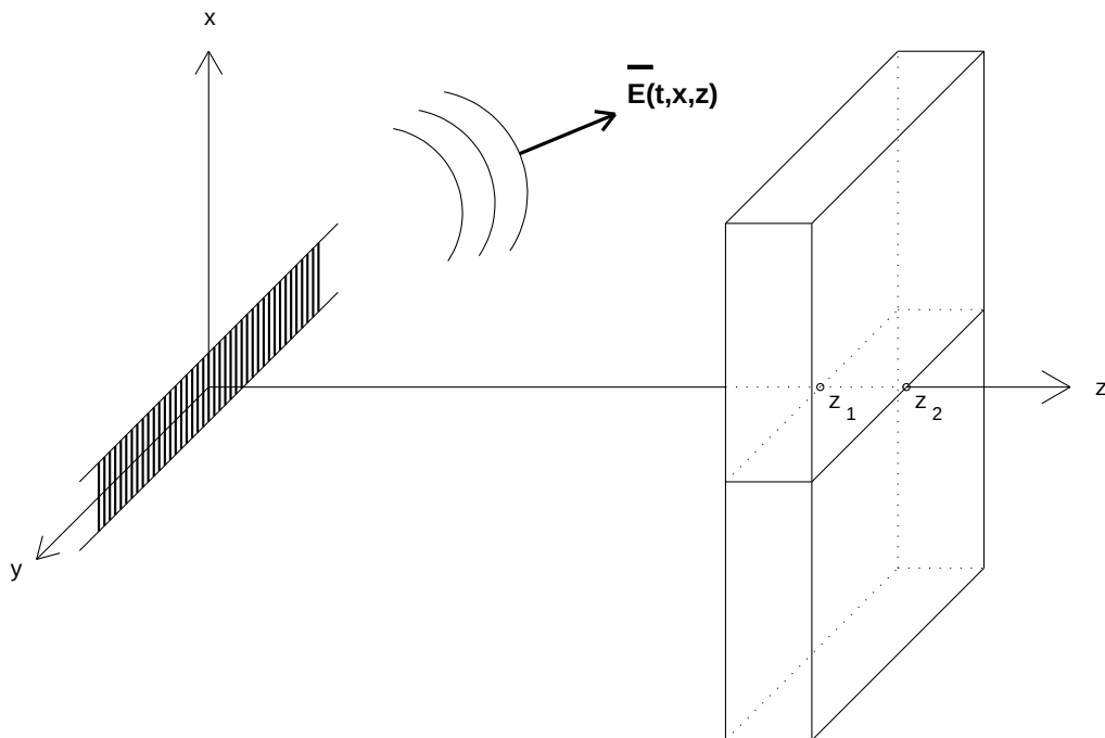
FIGURE 1. Antenna and dielectric material geometry
