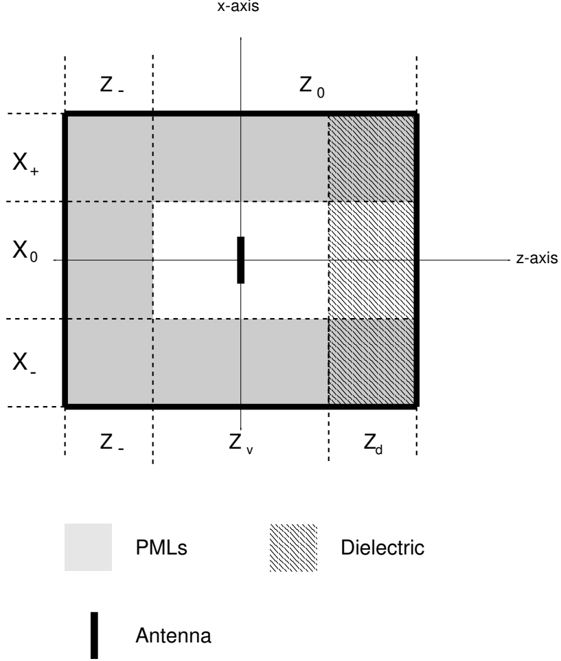
FIGURE 2. 2-D problem geometry
