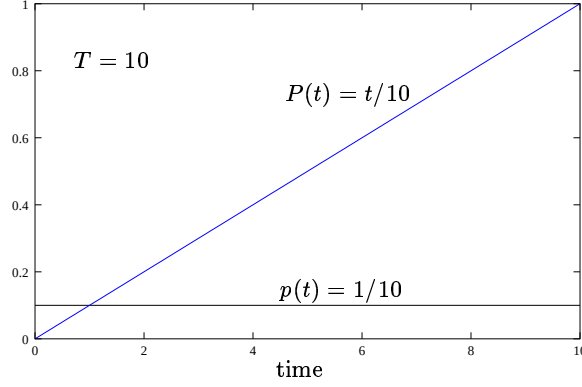
Figure 2.5: Uniform Distribution.
