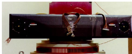
Figure 7. Random Vibration Tests
