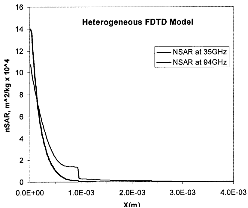
Figure 3. Normalized SAR values were calculated as a function of depth into the tissue for a 3-layer model of the rat skin.
