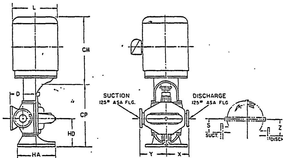
PUMP DIMENSIONS
