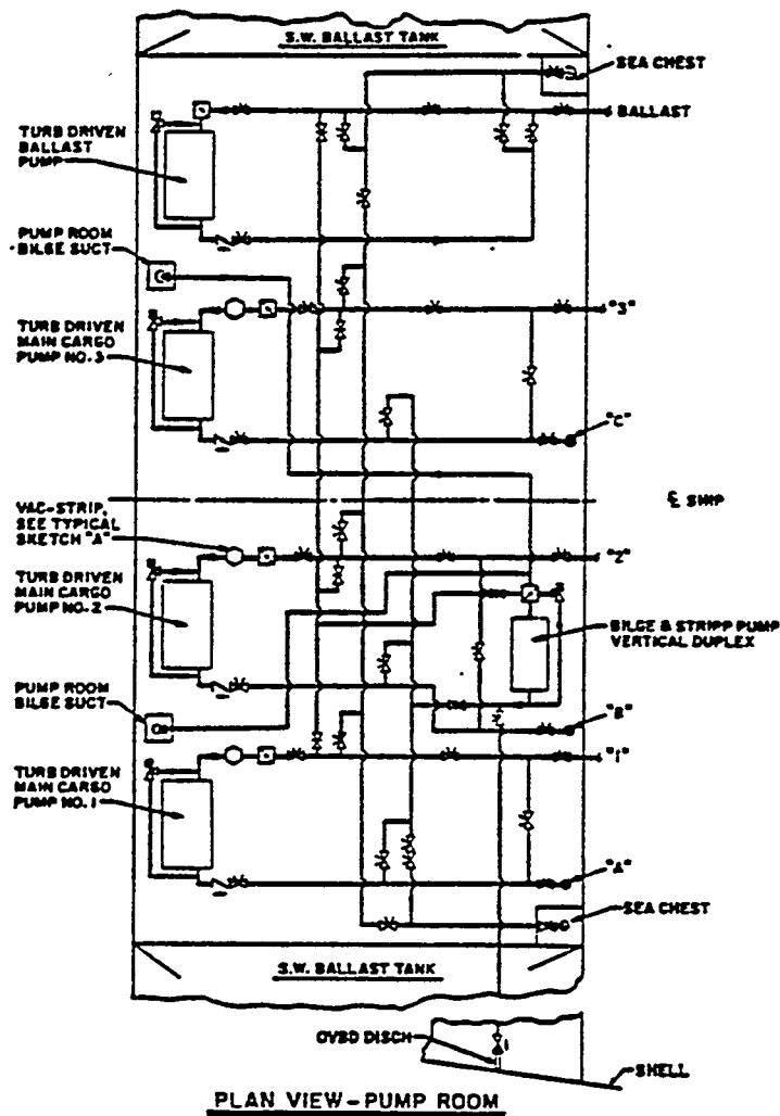
TYPICAL DIAGRAMMATIC ARR OF STRIPPING SYSTEM FOR CARGO OIL PUMPS
