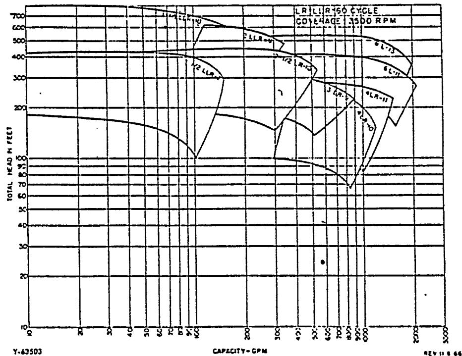
COMPOSITE CHARTS FOR TYPE LR, LLR PUMPS 3500 RPM - 60 CYCLE
