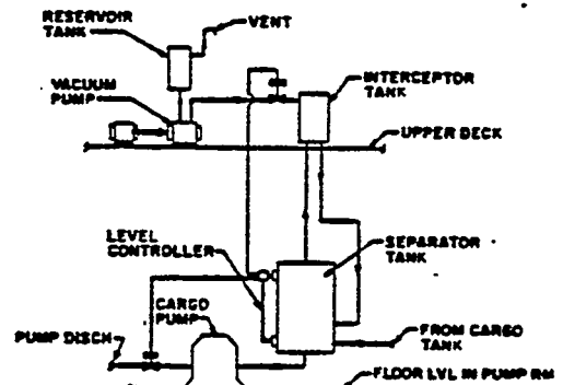
TYPICAL DIAGRAMMATIC ARR OF STRIPPING SYSTEM FOR CARGO OIL PUMPS
