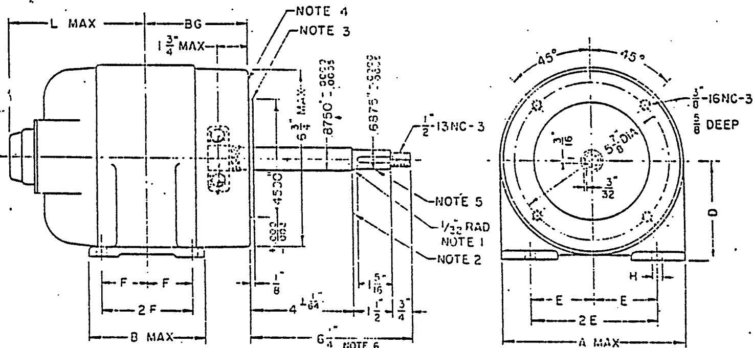
STANDARD FRAME DIMENSIONS AND BEARING SIZES FOR FRACTIONAL HORSEPOWER CLOSE-COUPLED MOTORS DIMENSIONS IN INCHES
