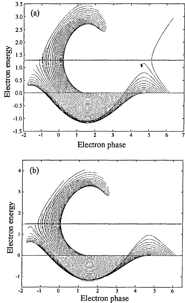
FIG. 4. Electron trajectories in the phase space "electron energy vs electron phase" in the clintotron with \tilde{\alpha}=0.1 (a), and \tilde{\alpha}=0.2 (b); the normalized initial detuning and the normalized interaction length have optimal values in accordance with Fig. 3(c).
