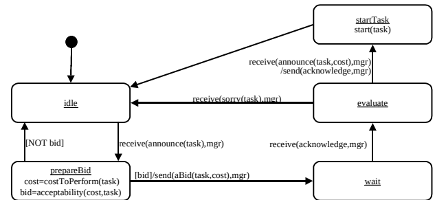
Figure 5: Contract Net Bidder Abstract Task
