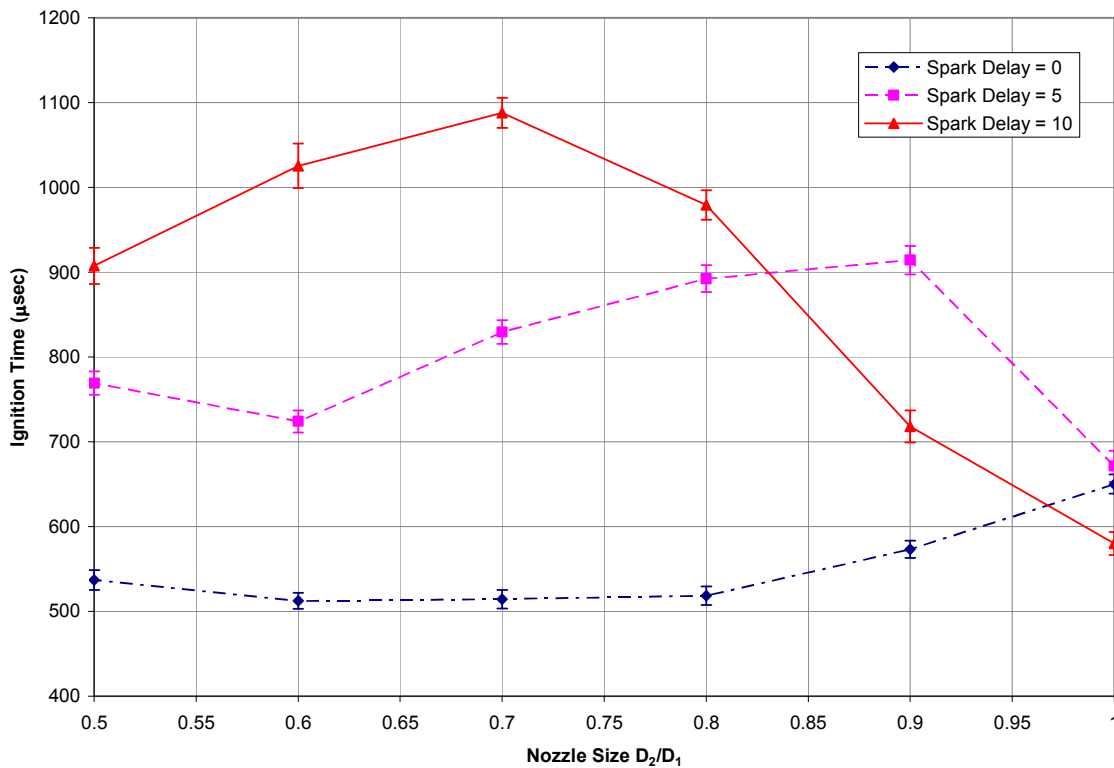
Figure 43. Ignition time versus nozzle size with varying spark delays ( FF = 2 , \phi = 1 )
