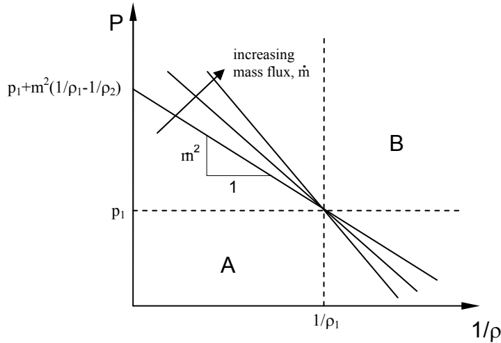
Figure 2. Rayleigh lines of constant mass flux
