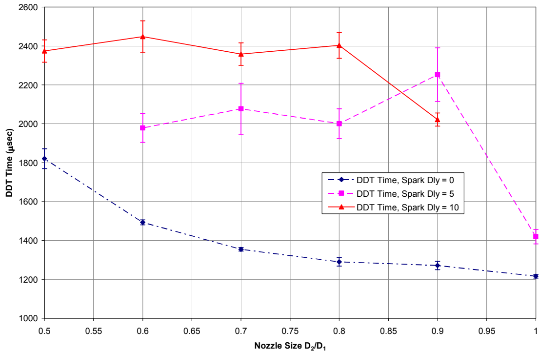
Figure 45. DDT time versus nozzle size with spark delay variation ( FF = 2 , \phi = 1 )
