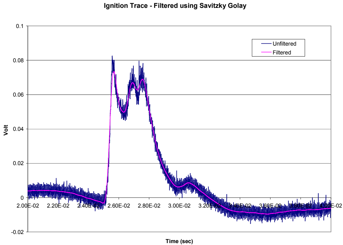
Figure 22. Ignition trace processed with Savitzky-Golay filter
