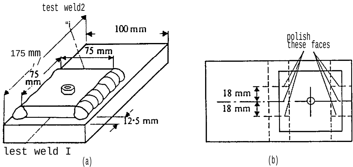
Figure 4. Configuration of Controlled Thermal Severity (CTS) test specimens.
