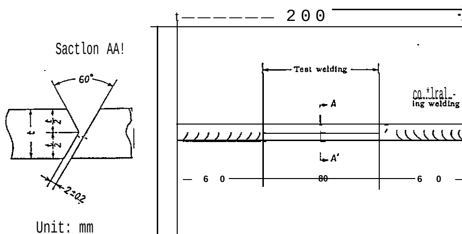
Figure 5. Configuration of Tekken test specimens. (From Japanese Industrial Standard JIS Z 3158 (1983).)
