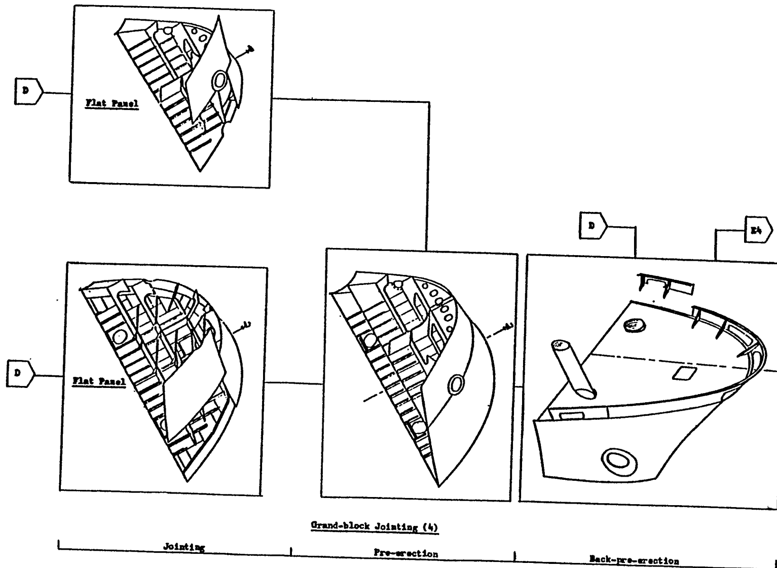
Figure Grand-block Jointing - Grand-block of Fore'side and Upper Deck of Fore Body
