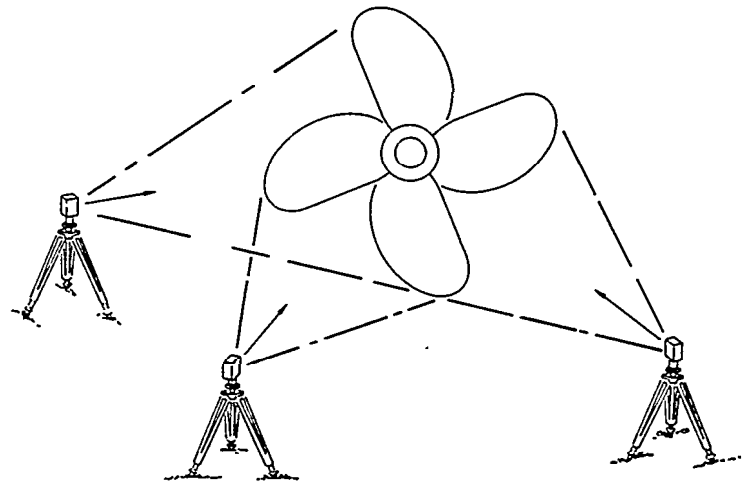
FIGURE B-5: Illustrating Convergent Photography. Camera axes are purposely inclined to one another and with respect to the scene. A single camera may be used to take all photographs.
