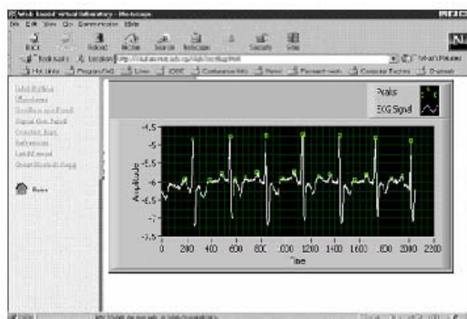
Figure 4 Displayed Cardiac signals using Lab view software
