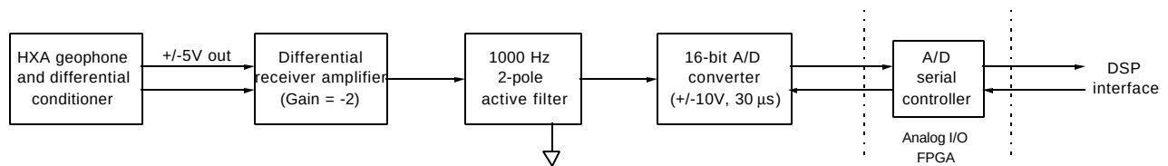
Figure 20: Input from geophone motion sensors to DSP
