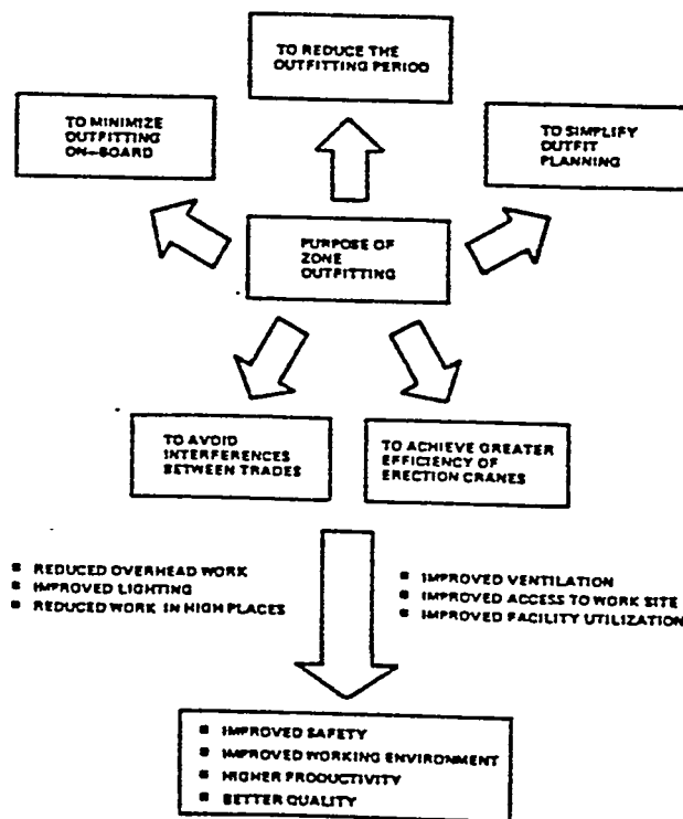
Figure I-2: Goals and Benefits of Zone Outfitting
