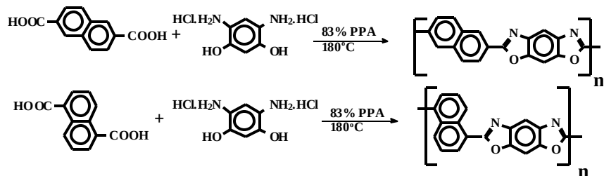
Figure 2. Synthesis of poly(benzobisoxazole)s with naphthalene-2,6-diyl and naphthalene-1,5-diyl structural units
