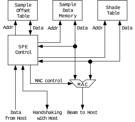
Figure 1: Beamforming Processor Block Diagram
