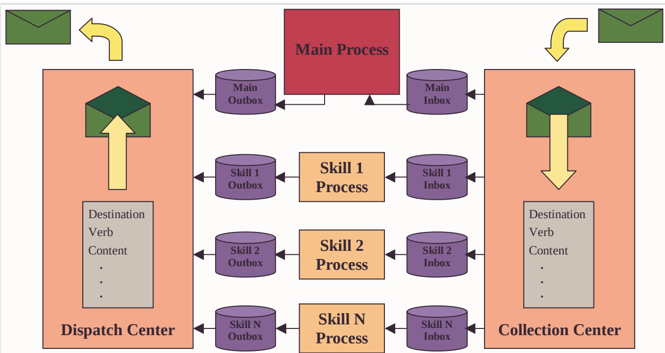
Figure 1. C++ Agent Architecture
