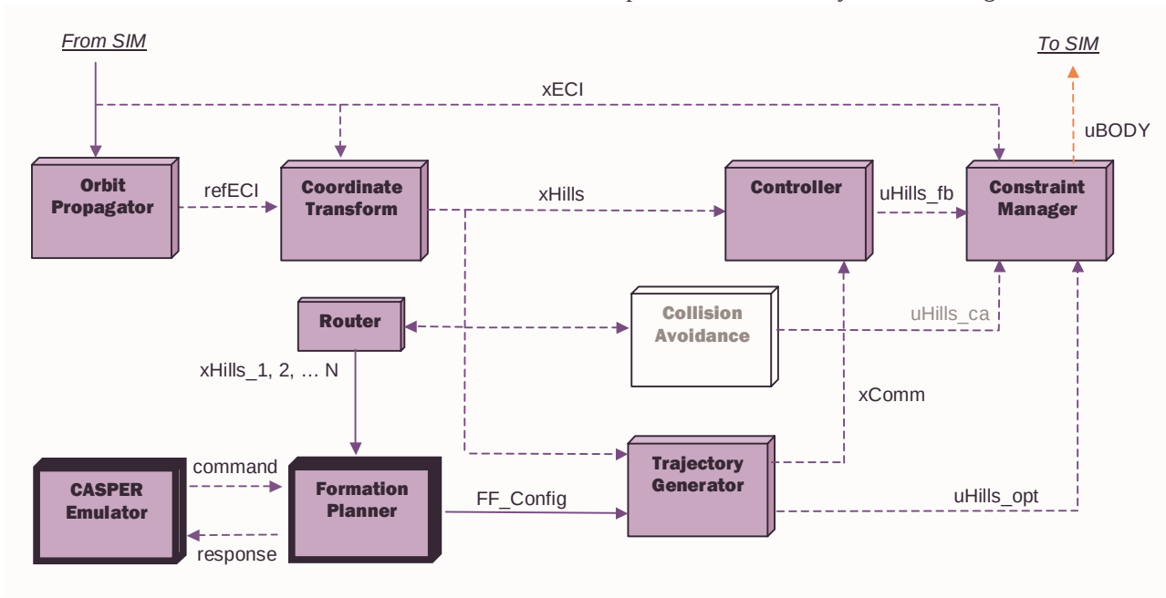
Figure 2: Cluster Manager Block Diagram
