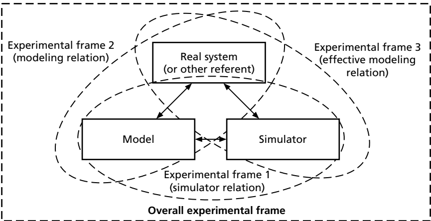
Figure A.1 Validating a Model Within an Experimental Frame
