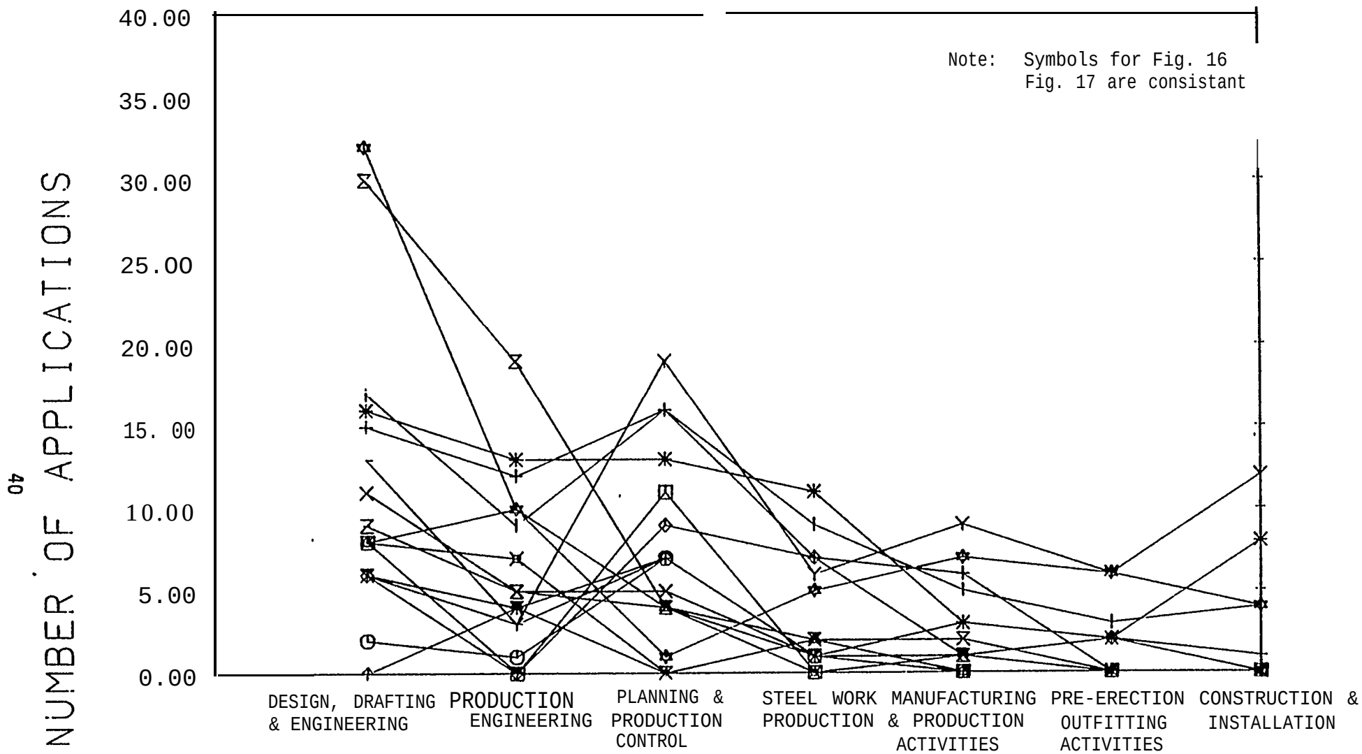
Figure 17. Functional Applications by Shipyard
