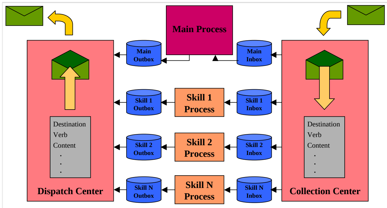
Figure 4. C++ Agent Architecture
