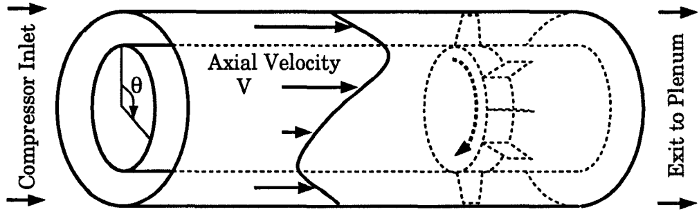
Figure 6.1: A schematic of the compressor geometry
