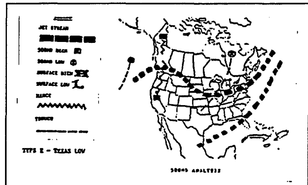
Texas Low 500 MB Pattern
