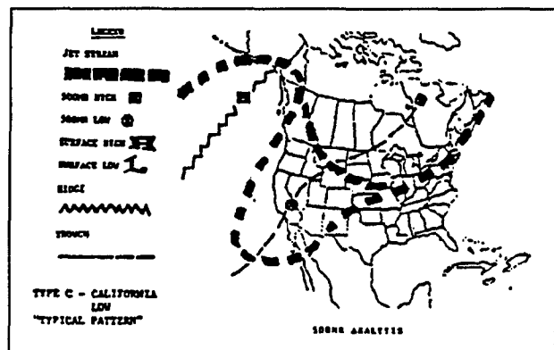
California Low 500 MB Pattern
