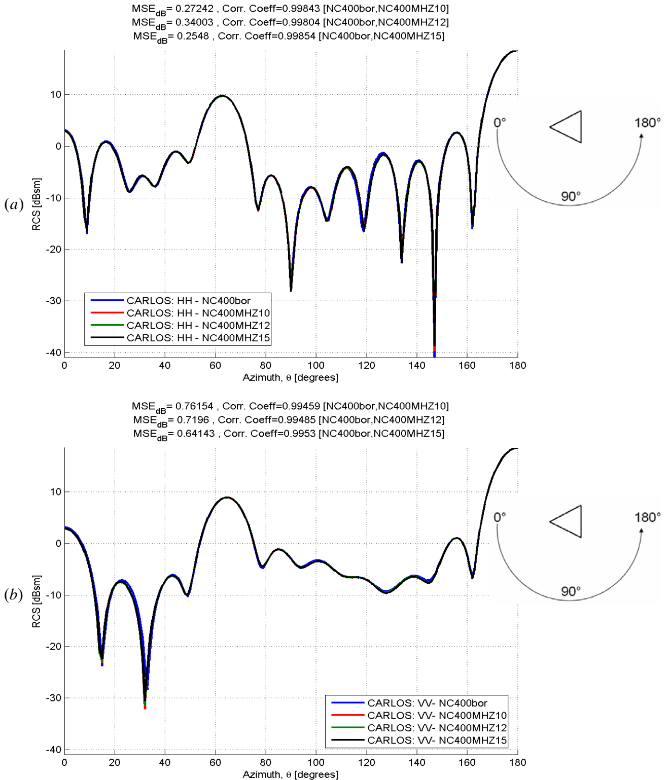
Figure 4-8: CARLOS RCS prediction of the missile nosecone showing convergence with increasing grid densities given in a) 400 MHz HH b) 400 MHz VV. Convergence is shown by reduction in MSE dBsm and increase in the value of the correlation coefficient
