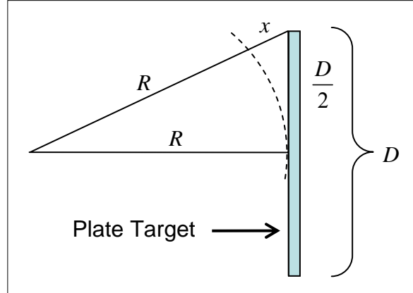
Figure 2-9: Cross-range phase variation
