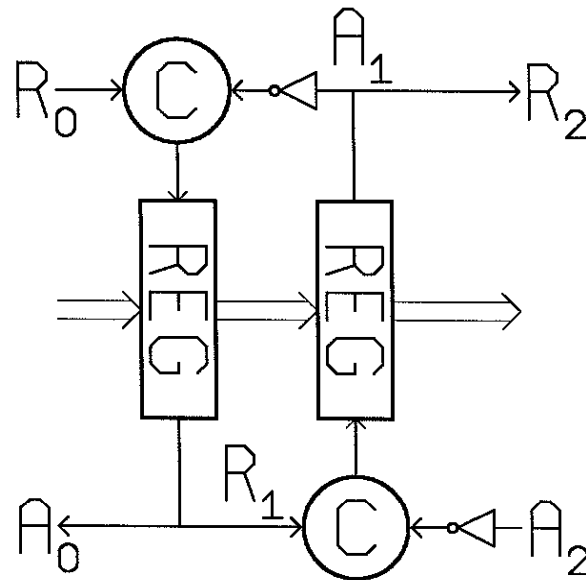
Figure 18: Asynchronous FIFO
