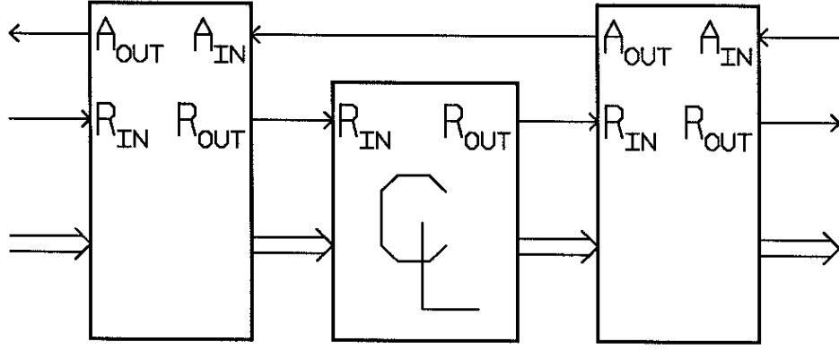
Figure 17: Asynchronous pipeline
