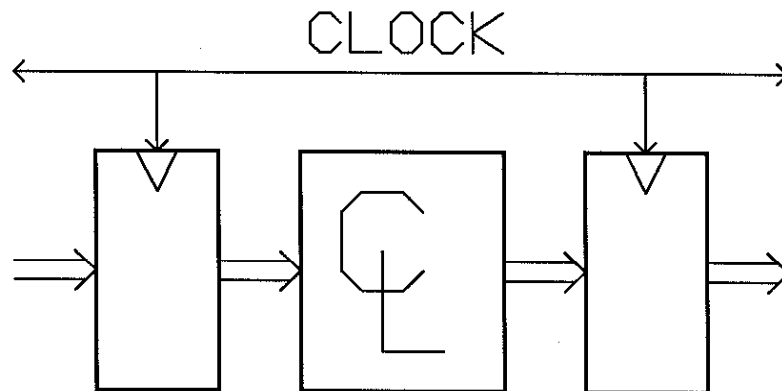
Figure 16: Synchronous pipeline
