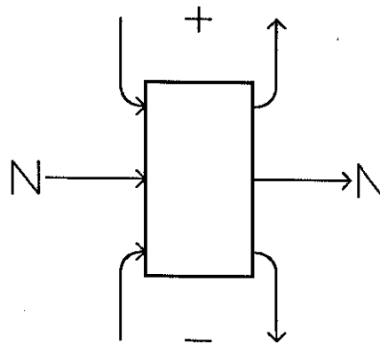
Figure 5: 1-D automaton
