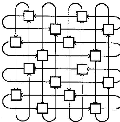
Figure 2: Torus network
