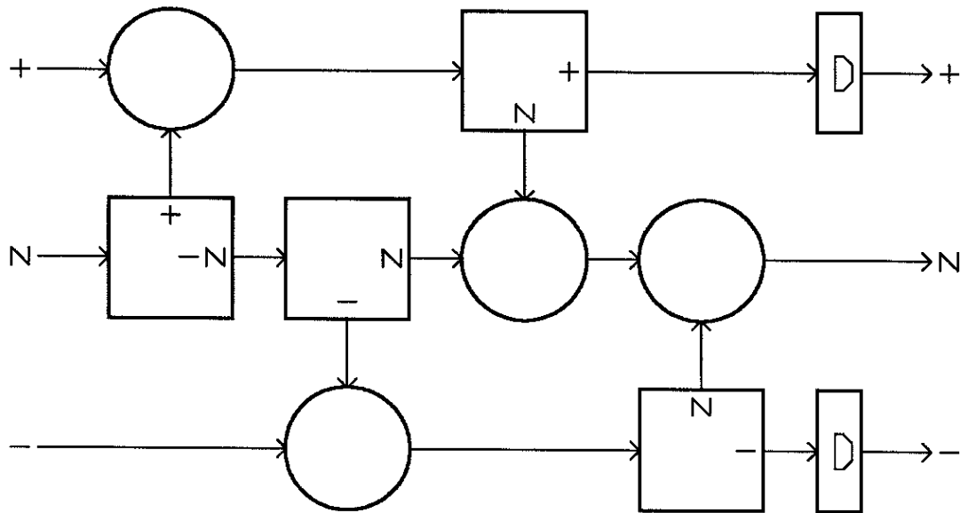
Figure 22: Asynchronous automaton
