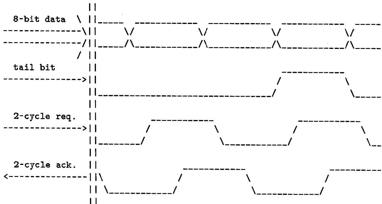
Figure 15: MRC signals and timing
