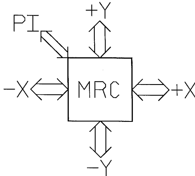
Figure 13: Mesh routing chip
