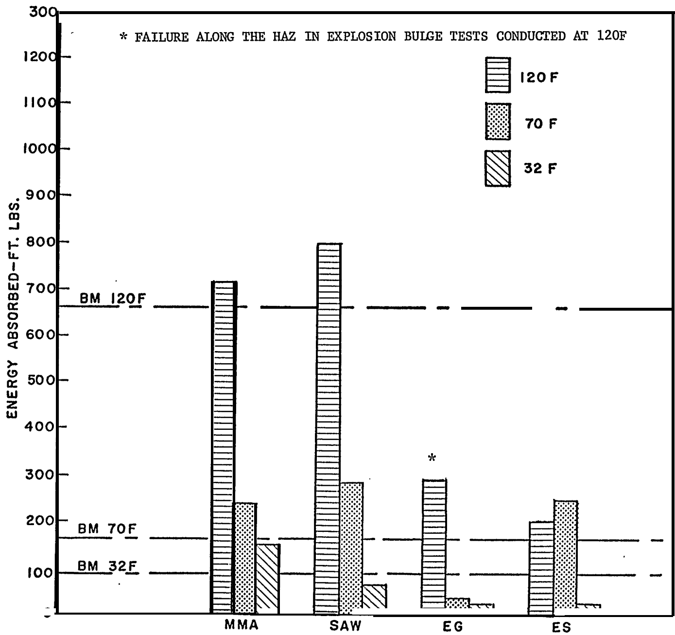
FIGURE 27 DYNAMIC TEAR HAZ TEST RESULTS
