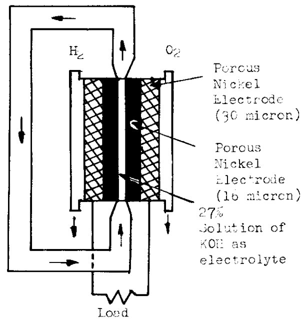
FUEL CELL
