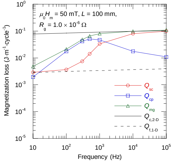
Fig. 3.6 (a) Losses vs. frequency (b) Losses vs. field amplitude Overall magnetization loss and loss components of multifilamentary YBCO coated conductor where R_g = 1 \mu\Omega .
