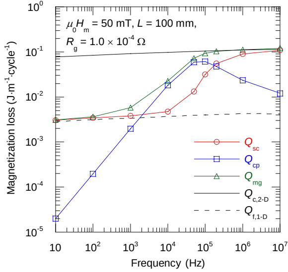
Fig. 3.7 (a) Losses vs. frequency (b) Losses vs. field amplitude Overall magnetization loss and loss components of multifilamentary YBCO coated conductor where R_g = 100 \mu\Omega .
