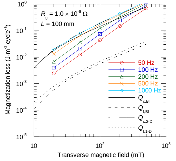
Fig. 3.6 (a) Losses vs. frequency (b) Losses vs. field amplitude Overall magnetization loss and loss components of multifilamentary YBCO coated conductor where R_g = 1 \mu\Omega .
