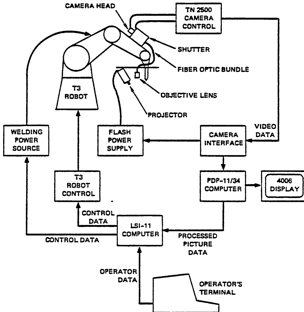
BLOCK DIAGRAM OF VISUALLY GUIDED ROBOT ARC-WELDING SYSTEM
