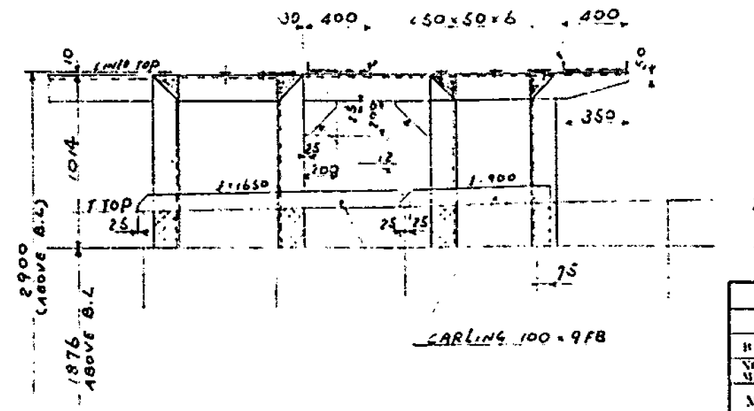
FIGURE 8-7: Typical Work Instruction for Fabricating an Auxiliary-Machinery Foundations.
