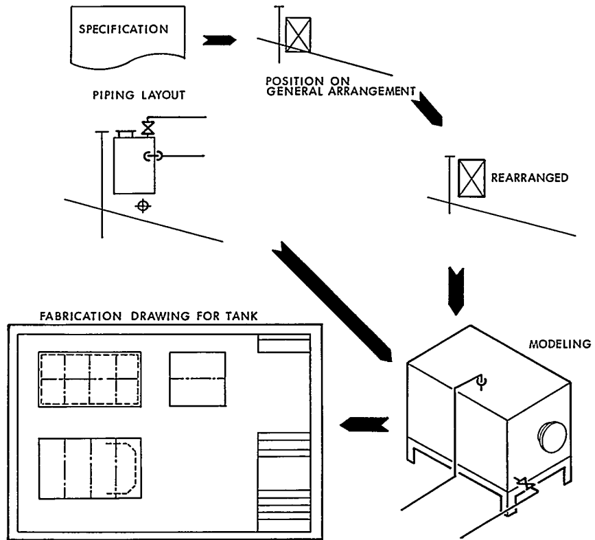
FIGURE 3-26: Design Modeling a Tank.
