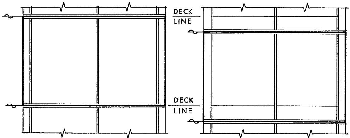
ELEVATIONS
