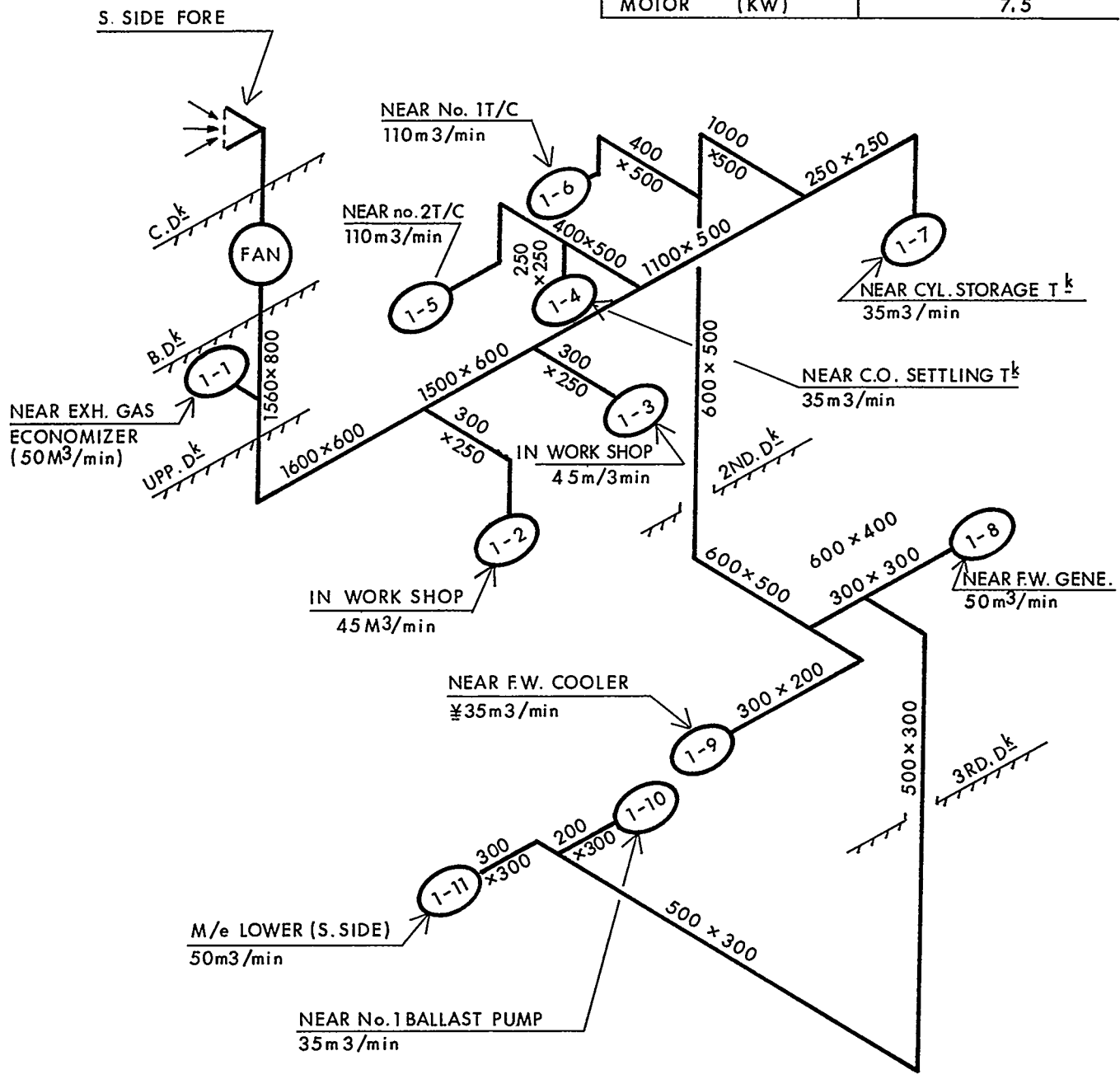
FIGURE 3-23: Diagram for an Engine-Room Ventilation System.
