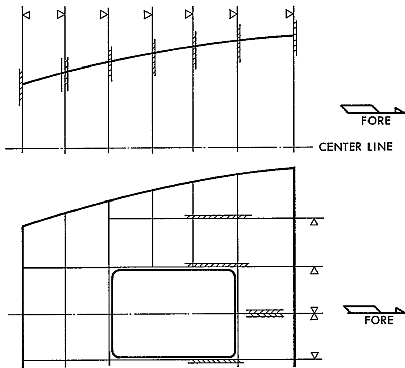
FIGURE 4-3: Reference Lines for Dimensioning (Plan Views).
