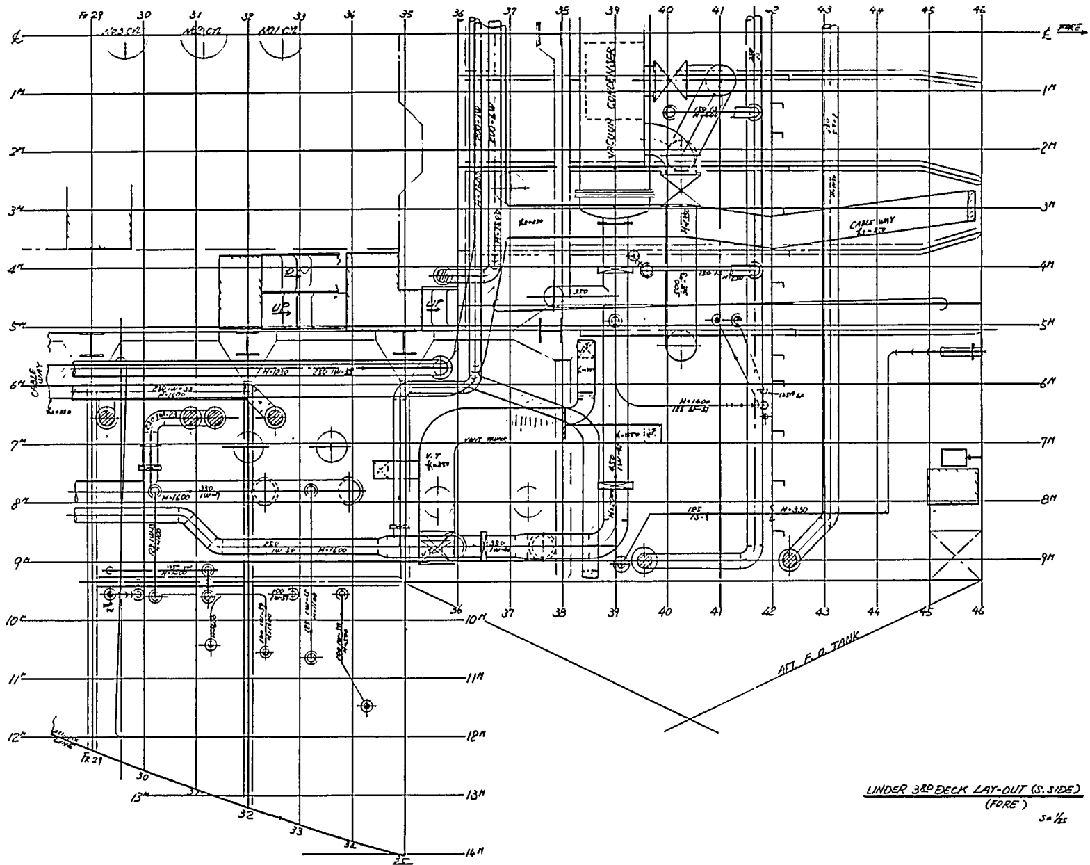
FIGURE 3-29(b): Rough Layout for an Engine-Room (Under 3rd Deck).
