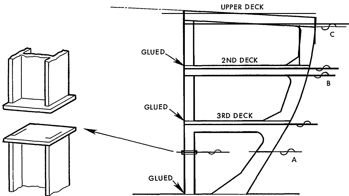
FIGURE 4-21: Attaching Columns. The division shown at A corresponds to that for erection of the actual hull. The divisions at B and C are only to facilitate assembly and disassembly of the model.
