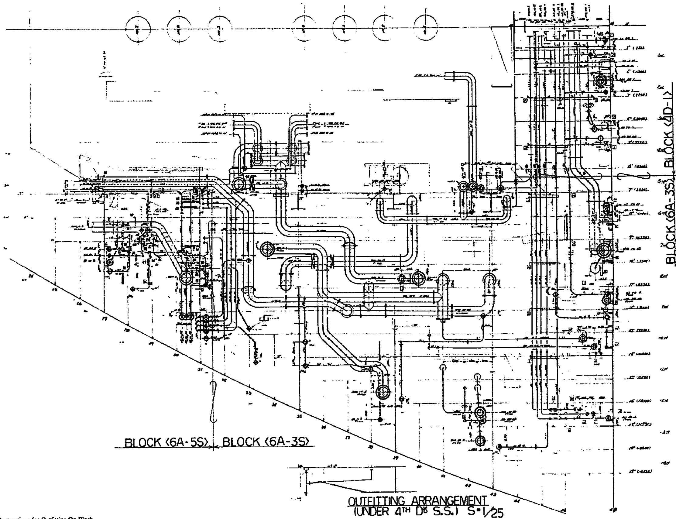
FIGURE 8-3: Typical Work Instructions for Outfitting On-Block.
