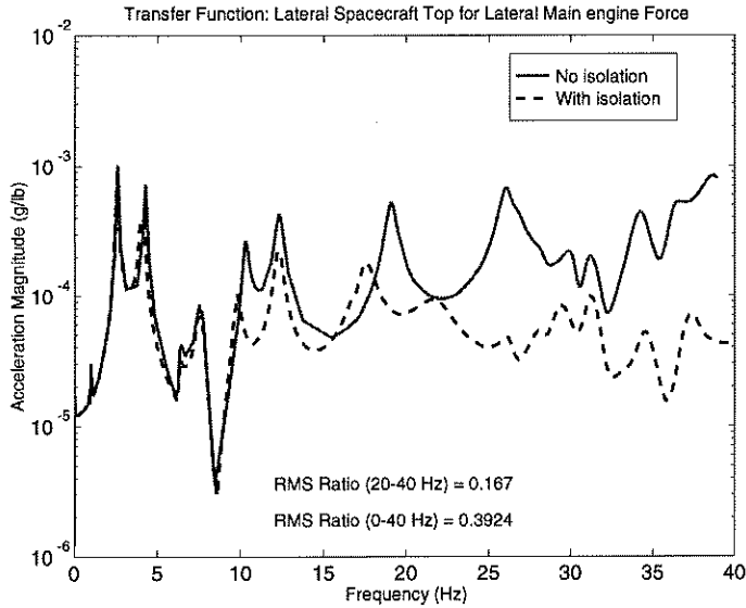
Figure 5: Transfer function showing lateral isolation
