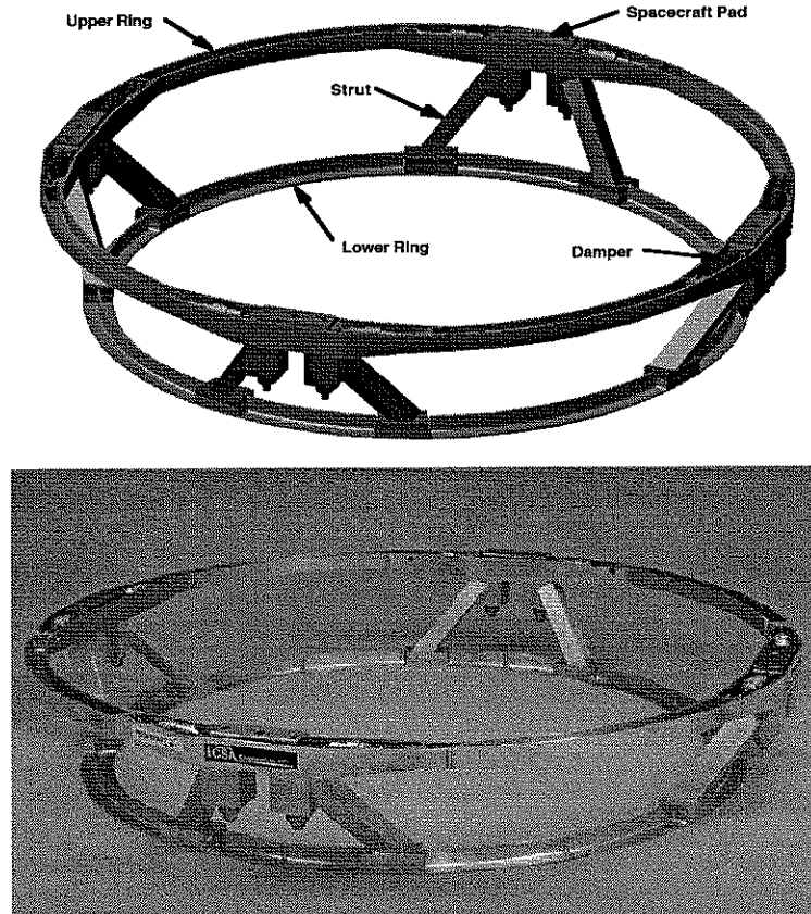
Figure 6: PIP isolating payload attach fitting: solid model and full-scale hardware (69" diameter)
