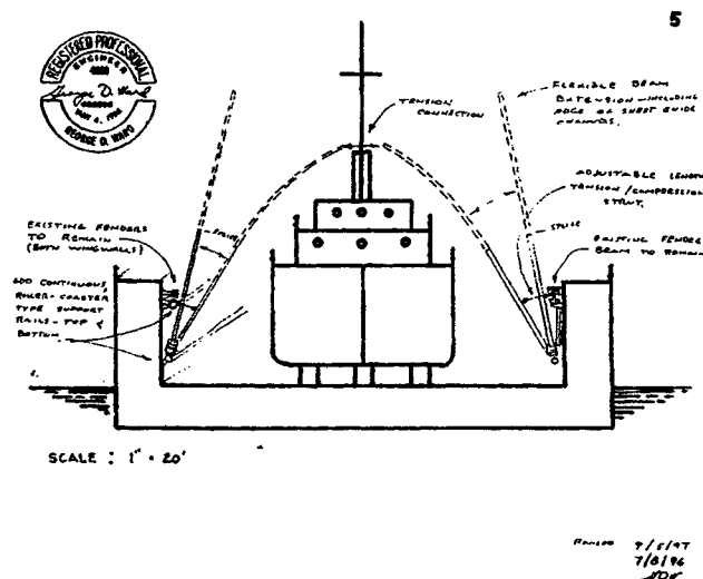
Figure 29 Combination Inflexible & Flexible Booms Cantilevered to Closed Position
