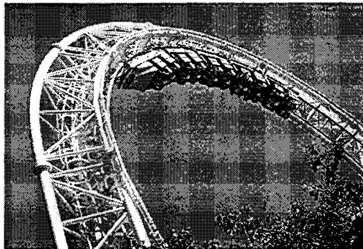
Figure 6: 3-Chord Truss
