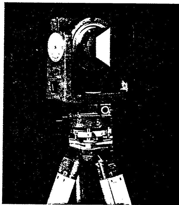
FIGURE 2-5: The Wild P31 Universal Terrestrial Camera. This model accepts single glass or film frames, is focusable over a range of distances and has a distortion-free lens. The camera is often used detached from the yoke/tripod assembly.
