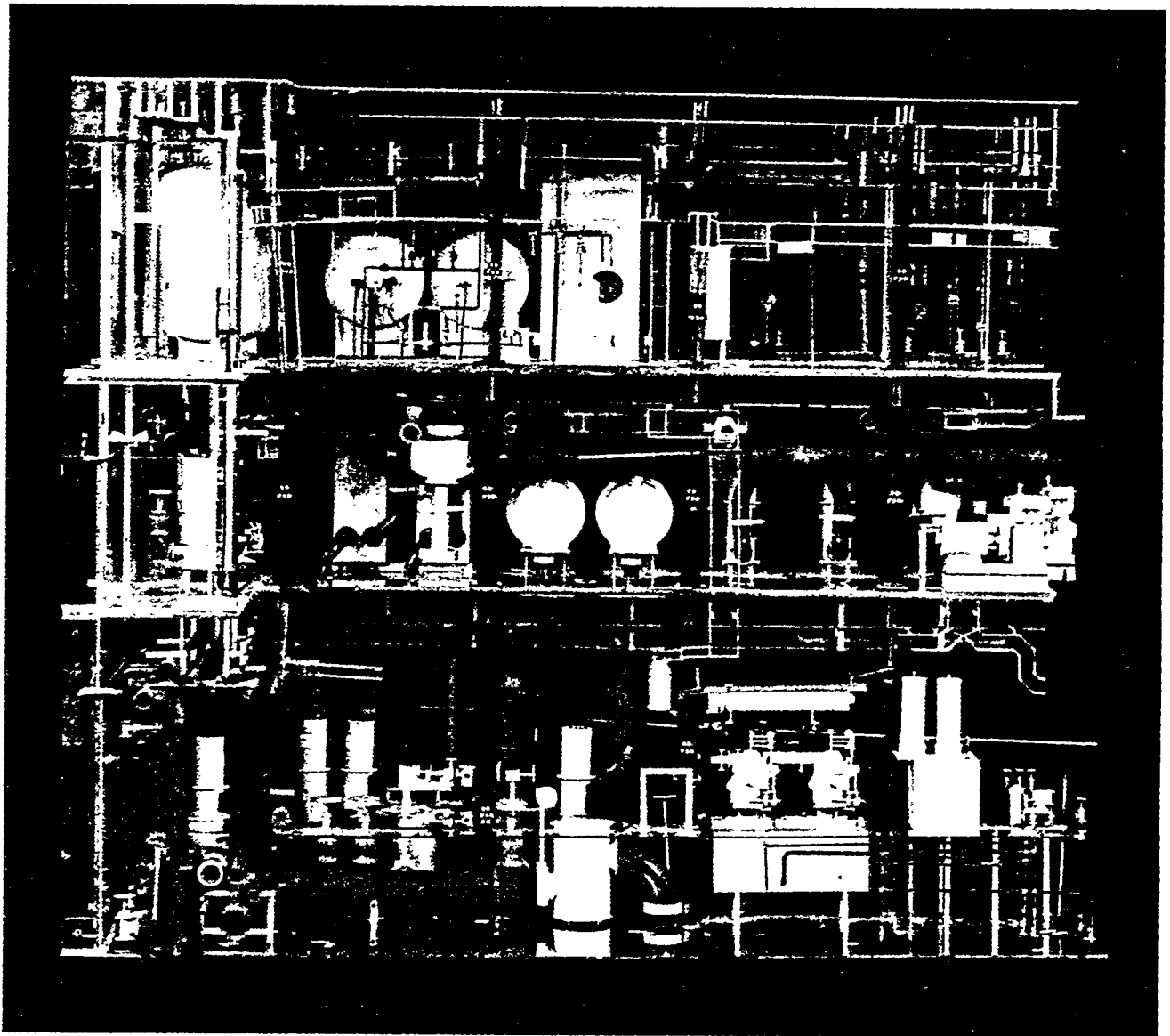
FIGURE 1-4: Design Model of a Ship's Engine Room. This model, consisting of a stack of six separable sections, was built by designers in lieu of preparing fitting-arrangement drawings. It includes just the machinery, piping and fittings arranged starboard and outboard of a main-propulsion diesel engine for an 18,930 DWT container ship. The model was used for final test of a developed system for photogrammetric dimensioning. Although this 1:15 scale model was built in Japan, many of its components were procured from Engineering Model Associates, Inc., City of Industry, California.
