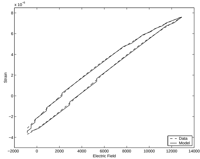
Figure 4. Experimental data from the stacked actuator and model prediction.
