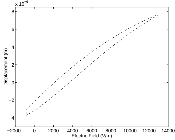
Figure 3. Relation between the input field E and displacements generated by a stacked PZT positioning mechanism in an AFM.
