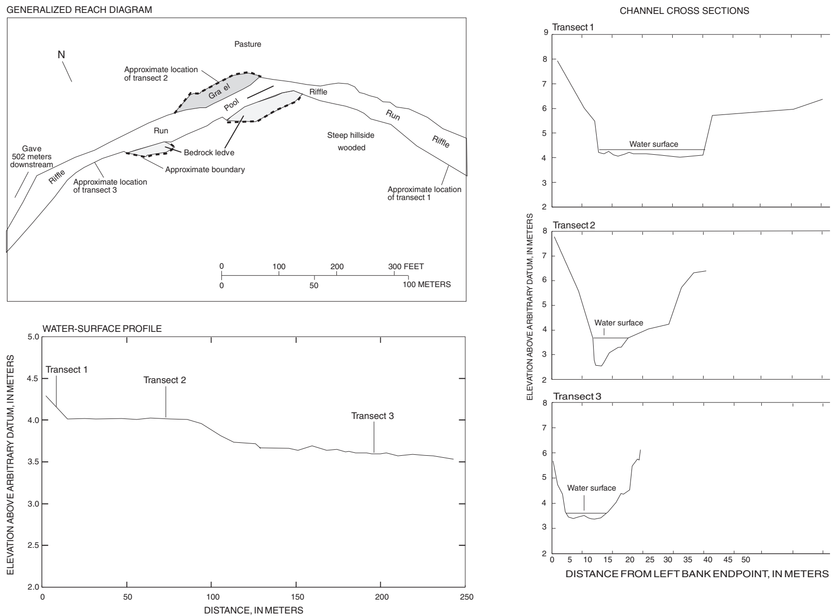
Figure 12. Generalized reach diagram, water-surface profile, and channel cross sections of Yocum Creek near Oak Grove, Arkansas (station number 07053250).
