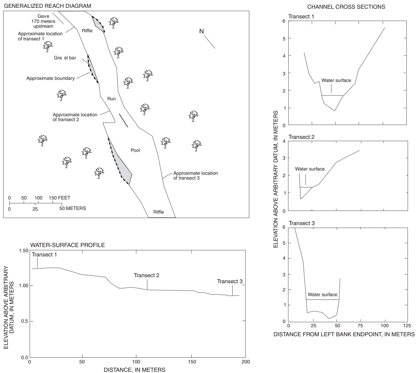
15 Figure 5. Generalized reach diagram, water-surface profile, and channel cross sections of the Niangua River at Windyville, Missouri (station number 06923250).
