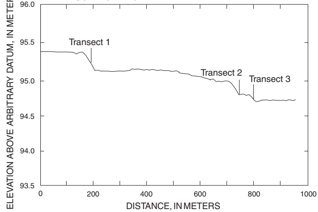
WATER-SURFACE PROFILE
