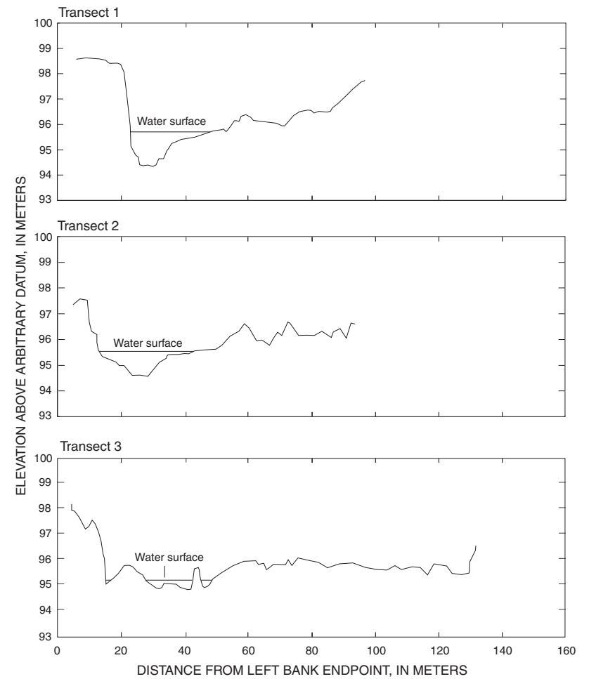
CHANNEL CROSS SECTIONS, 1994
