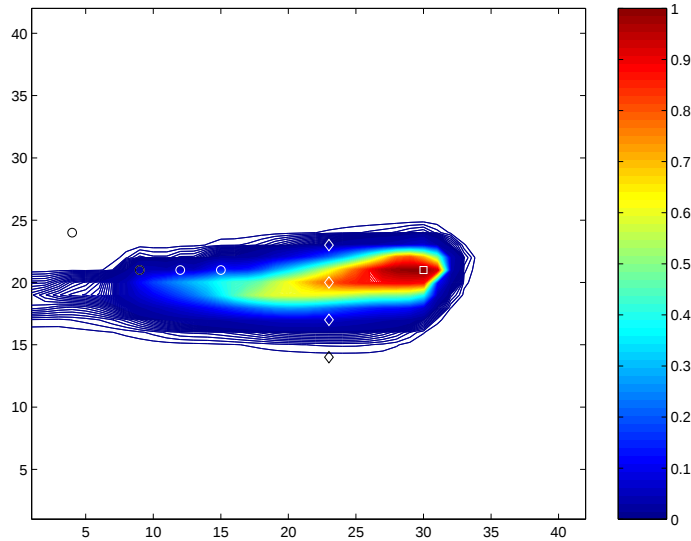
FIG. 4.1. Temperature Distribution: Uncontrolled Flow
