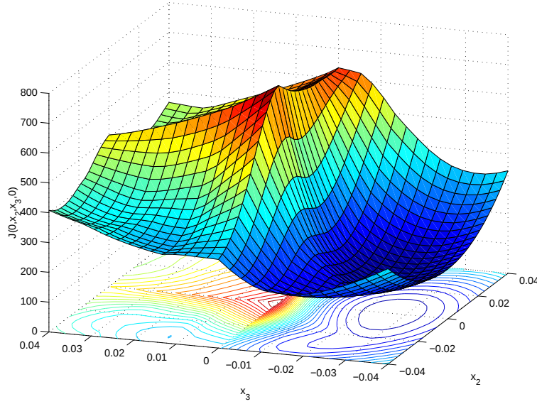
FIG. 1.1. Optimization Landscape
