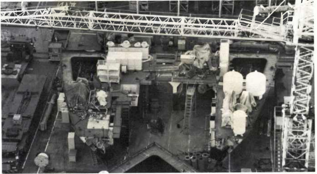
FIGURE 3-39: Or-bleck Outfitting Level. The right-side block is the same one shown in Figures 3-37 and 3-38. Zone and area are as described in Figure 3-37. Stage: on-floor fitting. This on-floor work is progressing next to the building dock. A light crane, of the type used for constructing buildings, is sufficient.
