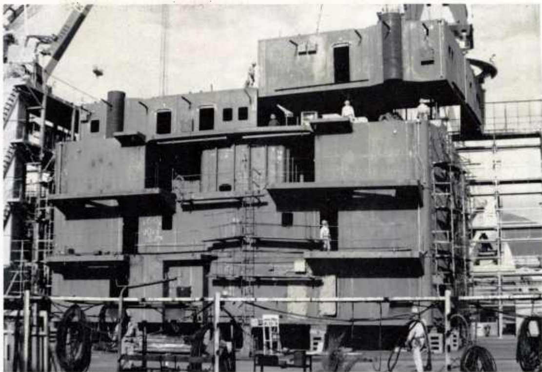
FIGURE 3-43: Grand-block Joining Level Zone: aft half of superstructure. Area: superstructure. Stage: pre-erection (this designates grand grand-block joining).
