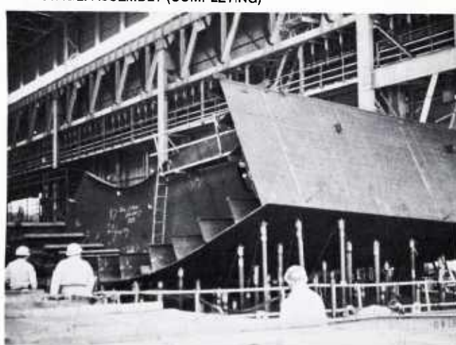
D. AREA: CURVED STAGE: ASSEMBLY
