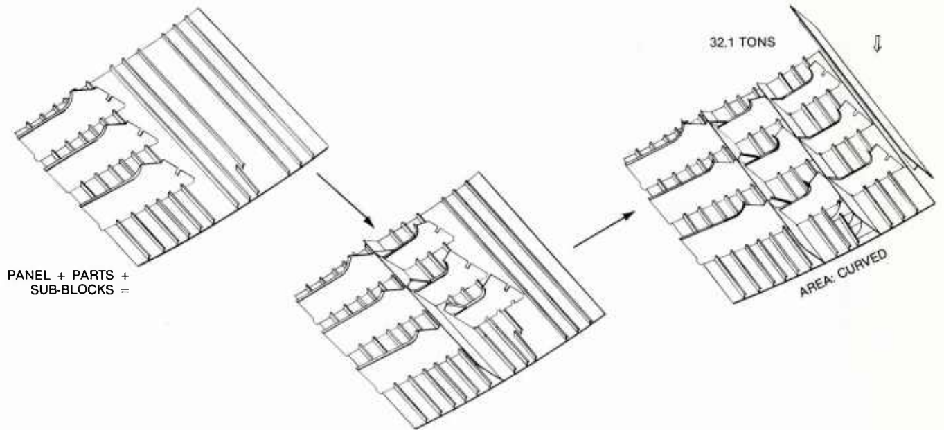
FIGURE 3-17: Block Assembly — Side Shell of Engine Room.
