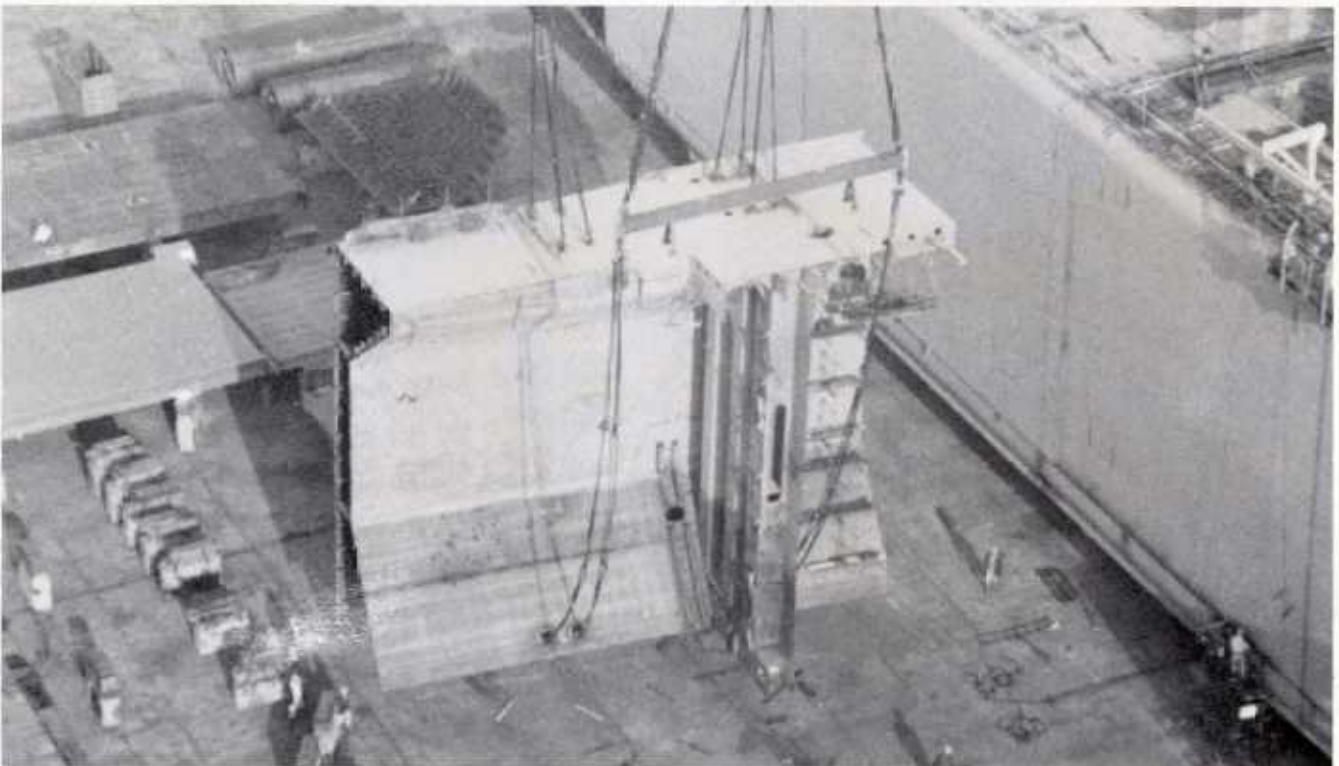
FIGURE 3-34: Same Grand Block as shown in Figure 3-33. The exposed shop primer, limited to the Transverse Hopper surface in this view, is in good condition.
