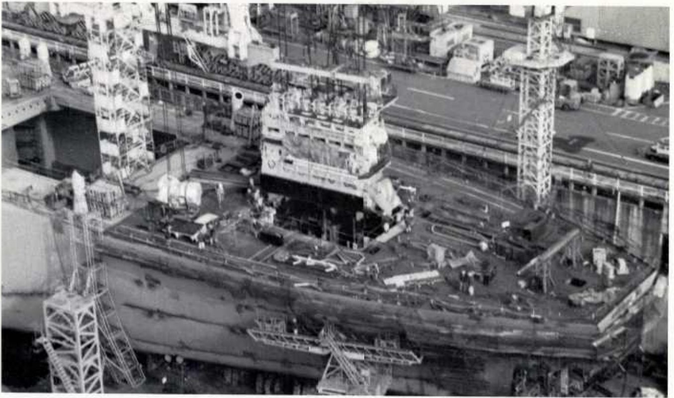
FIGURE 3-51: Erection Level. Landing the main engine. Stage: on-oper-space fitting (blue sky fitting). Keel laying plus 24 workdays.
