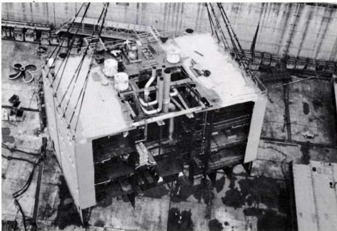
FIGURE 3-54: Erection Level. Aft half of superstructure being lifted. Finish under-coat painting has been completed on all vertical surfaces. Keel plus 29 workdays.
