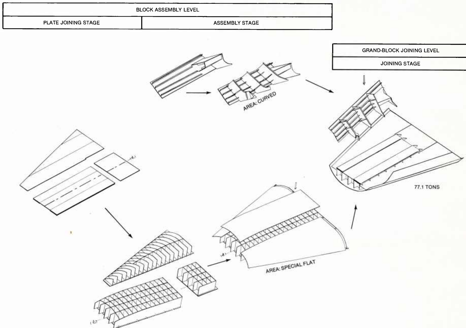
FIGURE 3-16: Block Assembly and Grand-block Joining — Bottom of Engine Room. The engine-room bottom block is classified by area as SPECIAL FLAT because of its work content and the projection of the main-engine foundation.
