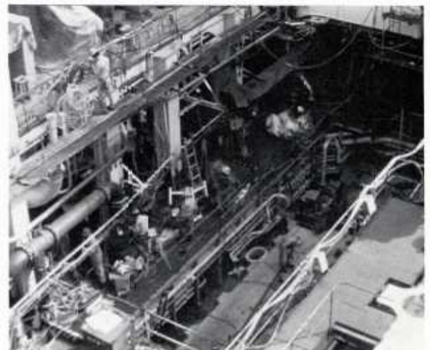
FIGURE 3-28: As much as possible, necessary outfitting is performed before the main engine is landed in order to facilitate access.
