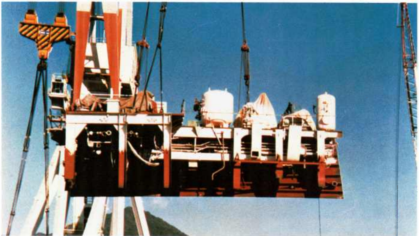
FIGURE 3-38: Same block as in Figure 3-37 after on-floor fitting and finish under-coat painting (white). The incomplete primer coat shown in Figure 3-37 was completed just after on-floor fitting when the lower structure was readily accessible.
