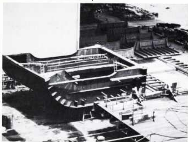
C. AREA: SPECIAL FLAT (NON-UNIFORM WORK CONTENT) STAGE: ASSEMBLY (OFF FLOW)
