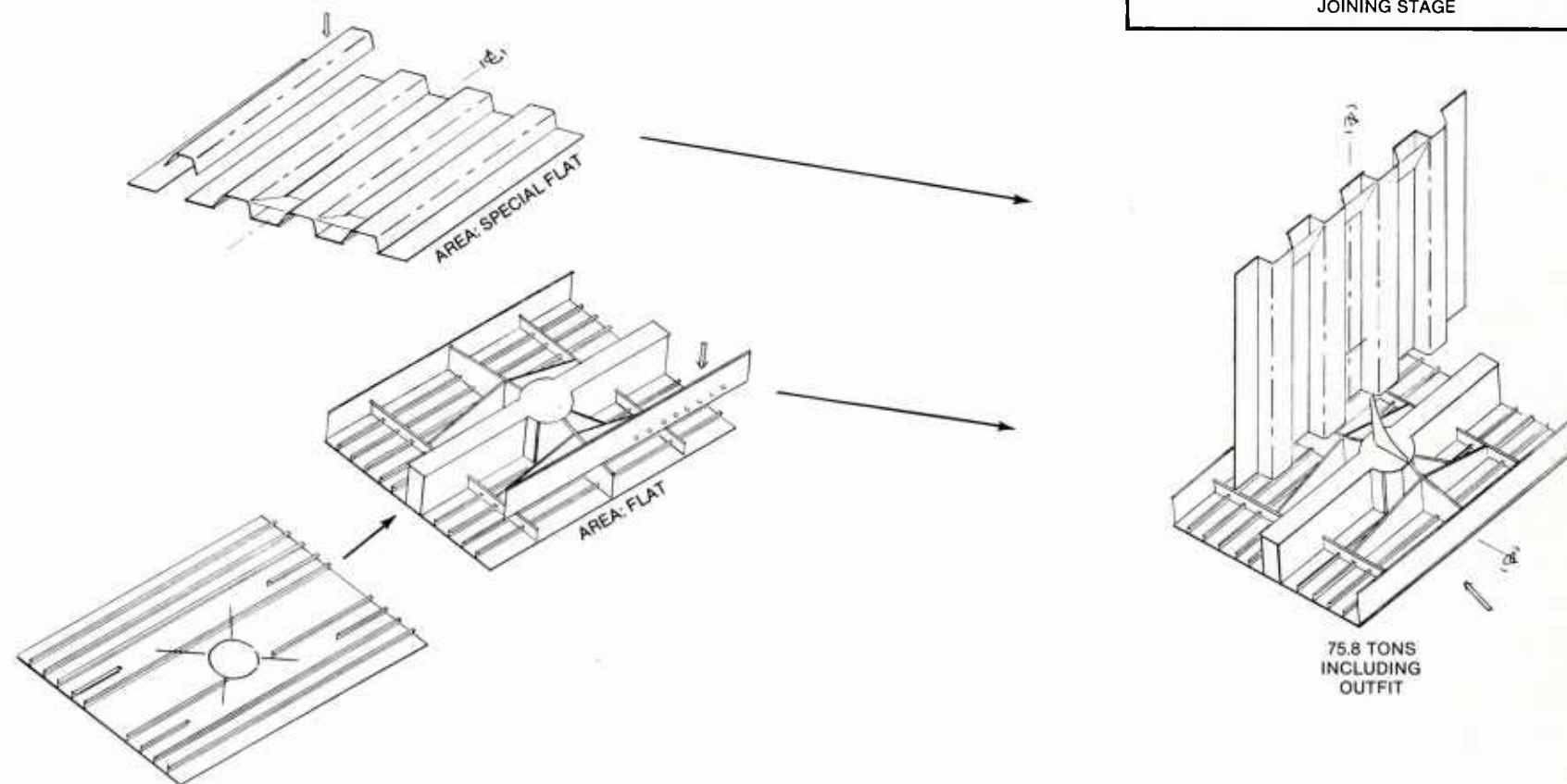
FIGURE 3-10: Block Assembly and Grand-block Joining. Corrugated Transverse Bulkhead and Deck Center Between Cargo Holds.
