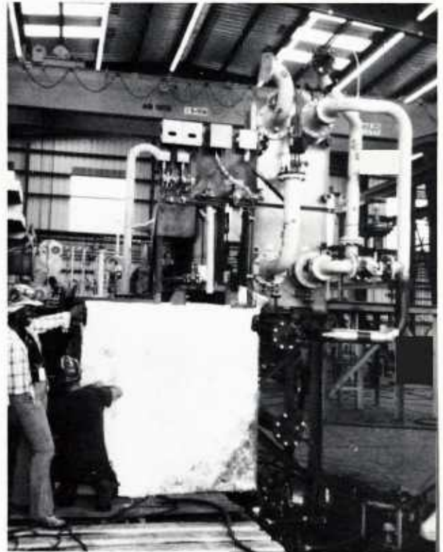
FIGURE 3-23: A tank, which is part of an engine-room unit, is being completely insulated in a unit-assembly shop. Portions of pipe systems incorporated are being hydrostatic tested at the same time.
