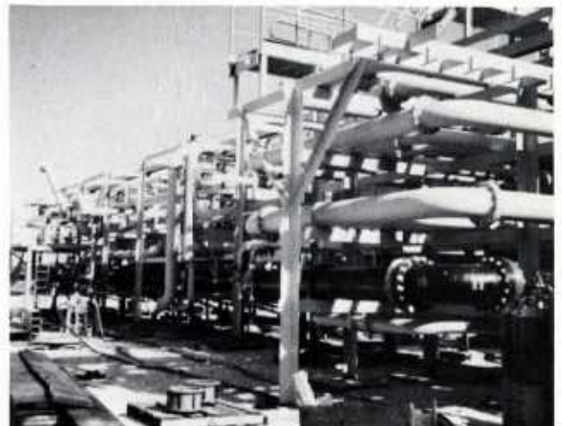
FIGURE 3-25: Very complex deck units for a product carrier, each 40 feet long, are assembled contiguously to insure that they will mate when landed on board. Upon completion the overall assembly will be about 400-feet long.
