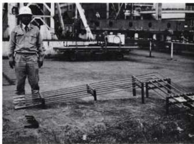
FIGURE 3-21: Unit sizes vary significantly. Top: Engine-room tank-tcp unit for a 100,000 deadweight-ton diesel-propelled tanker. Bottom left: Heat exchanger, foundations, pipe pieces, etc., incorporated as a unit. Bottom right: The author showing a small unit consisting of pneumatic tubing and supports.
