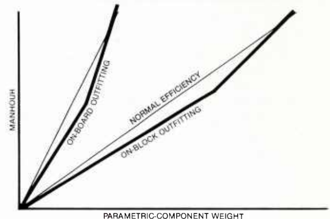
FIGURE 6-11: Productivity—Electrical Fitting of all components except cable. Each work package identifies total weight and parametric-component weight. The difference, i.e., items which comprise non-parametric-component weight, are treated as exceptions.
