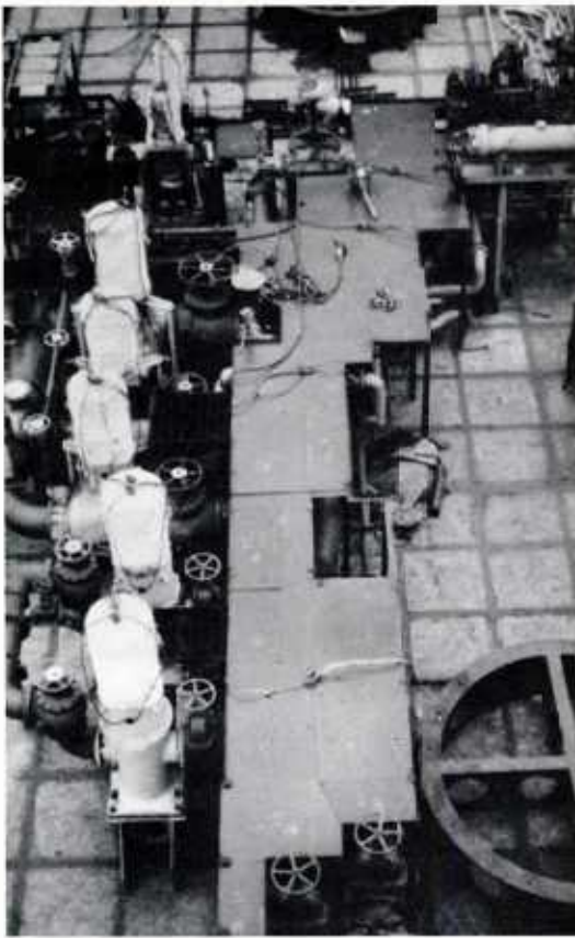
FIGURE 1-2: Outfit units which are dissimilar in arrangement and in functions incorporated, have the same classification in a product-oriented work breakdown structure because the problems associated with their assembly are the same.
