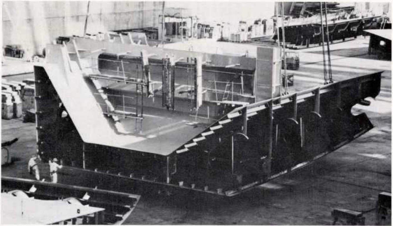
FIGURE 3-33. Grand Block of Side Shell, Top Side Tank, Transverse Hopper, and Side Transverse Bulkhead of Cargo Hold. Temporary staging is in place to facilitate erection welding. Primer has been applied to all surfaces except the bottom third which will be readily accessible after erection.
