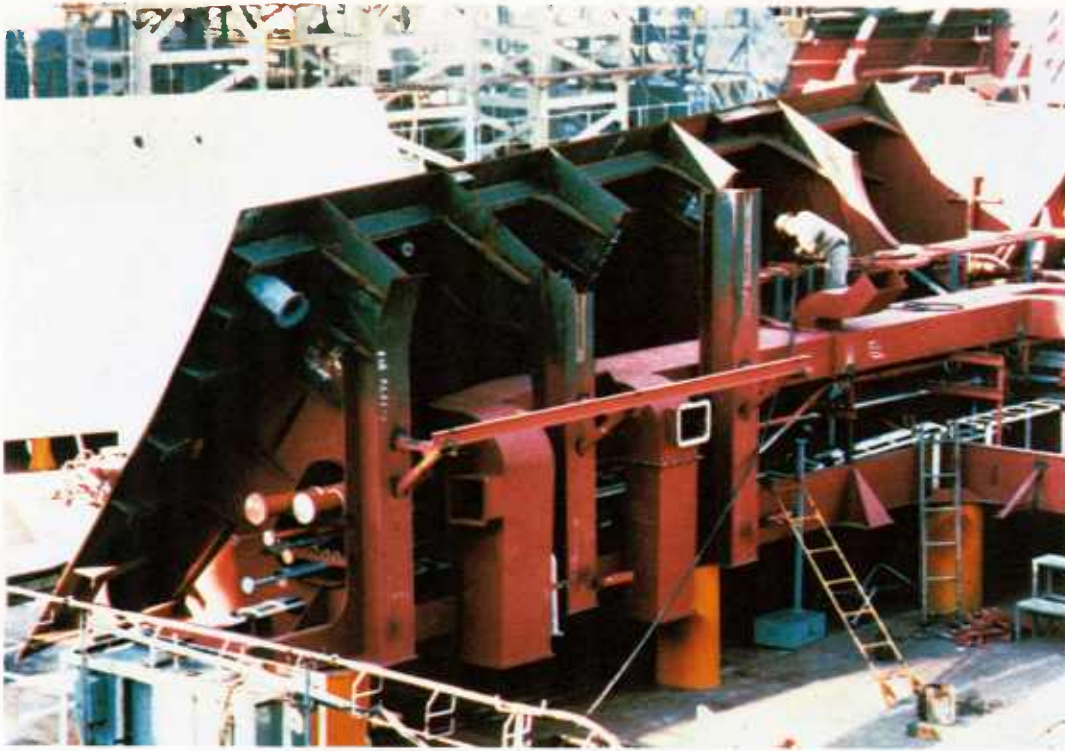
FIGURE 3-37: On-block Outfitting Level. Zone: region encompassed by side shell, engine-room flat and columns. Area: machinery components in large quantity (on flow). Stage: on-ceiling fitting. Before fitters started, red primer was applied to readily accessible structure. A primer coat was applied to individual pipe pieces, vent-duct pieces, etc., by their in-house or outside manufacturers.
