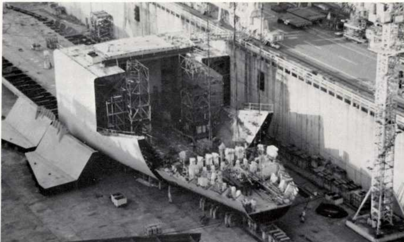
FIGURE 3-45: Erection Level. Landing the block shown in Figure 3-28. Keel laying plus 13 workdays.
