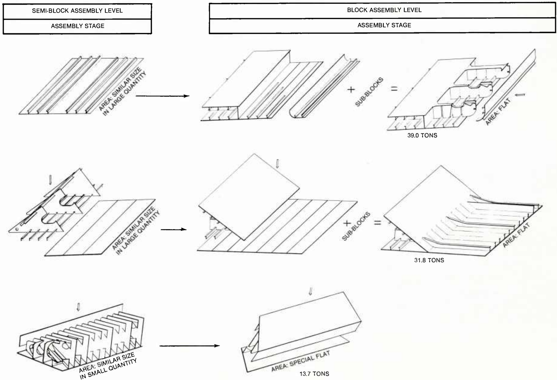
FIGURE 3-9: Semi-block and Block Assembly — Bottom Wing, Side Shell with Hopper, and Transverse Hopper in Cargo Hold. Problem area classifications SIMILAR SIZE IN LARGE QUANTITY and FLAT designate work for assembly lines (on-flow). SIMILAR SIZE IN SMALL QUANTITY and SPECIAL FLAT designate job-by-job work (off flow) because there are too few of them or because their work content is not uniform.
