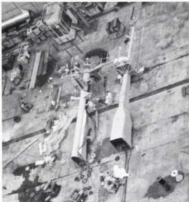
FIGURE 3-26: A Radar Mast and a Foremast with all components, including electrical, being assembled as units. Zone: unit. Area: large size unit. Stage: assembly. If the masts were hull-construction blocks, manufactured in-house, the fitting work would have been designated on block.
