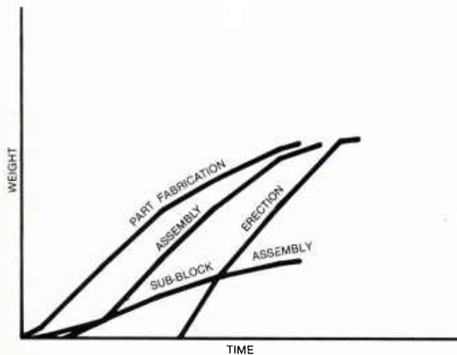
FIGURE 6-6: Production Progress—Hull Construction.
