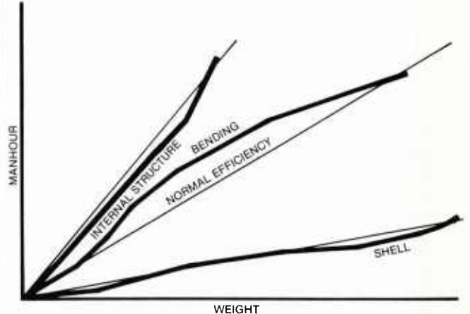
FIGURE 6-7: Productivity—Parts Fabrication. The plot for bending is by stage. The other two are by problem area. This illustrates the versatility of PWBS for fulfilling practical needs.
