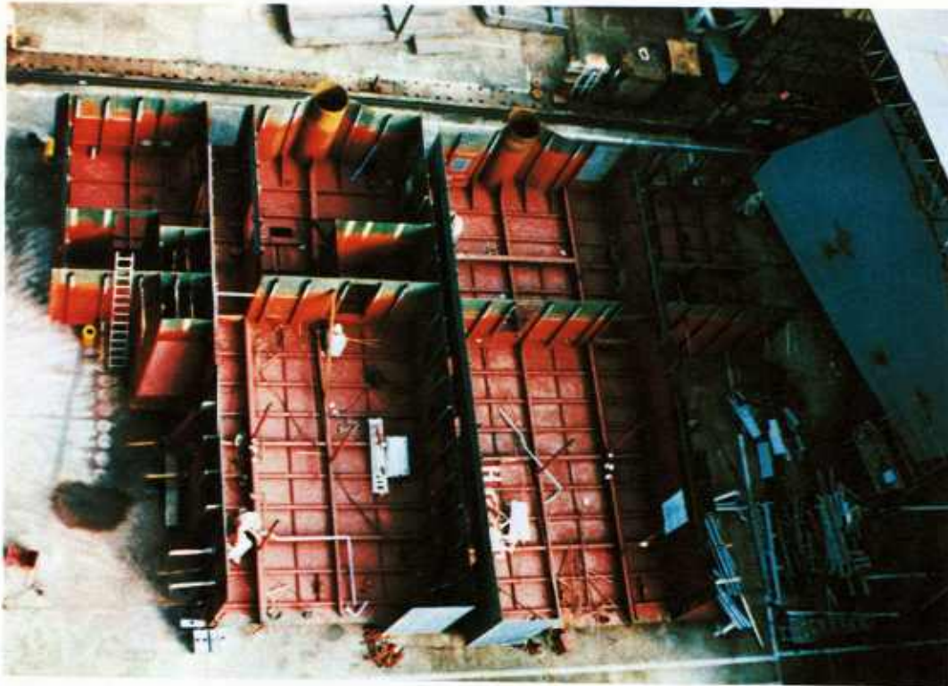
FIGURE 3-41: On-block Outfitting Level. Zone: two blocks, half of a superstructure deck. Area: accomodation components in large quantity (on flow). Stage: on-ceiling fitting. Red primer was applied just before outfitting started.
