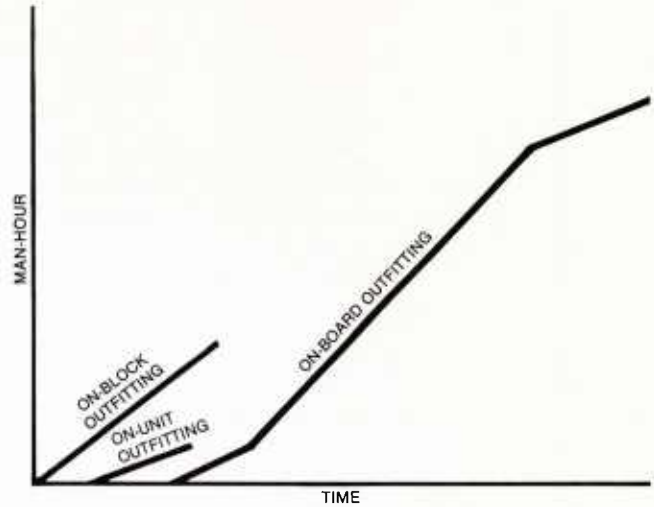
FIGURE 6-3: Manpower Expenditures—Machinery Fitting.
