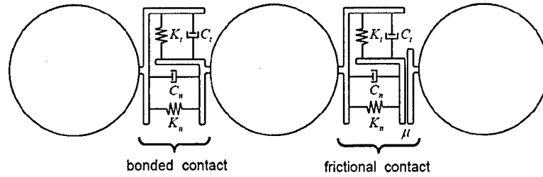
Figure 2.2 Discrete element interaction models for bonded and frictional contacts.
