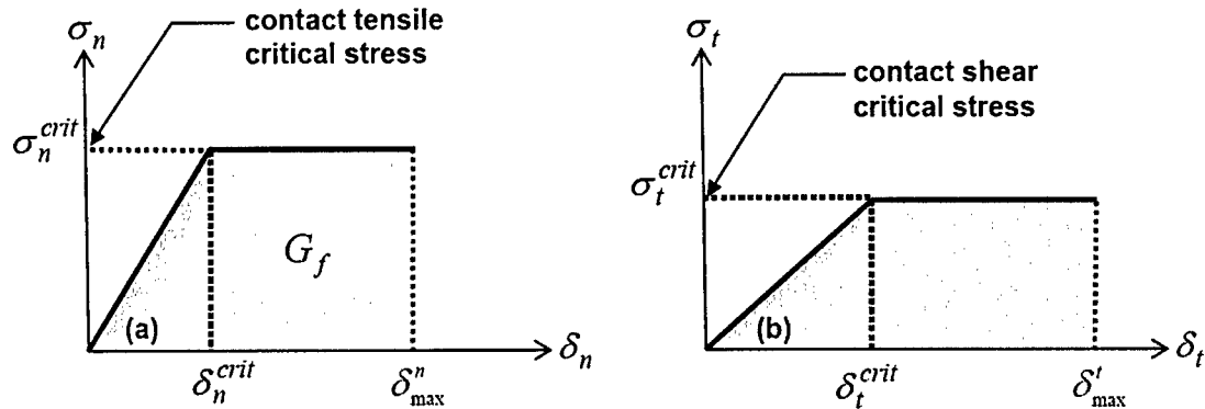
Figure 5.4 DEM contact stress-displacement behavior and fracture energy.
