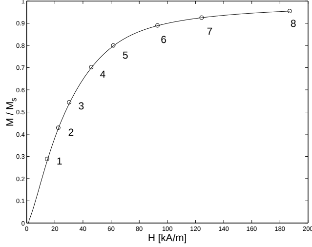
Figure 5: Initial magnetization curve showing the bias magnetization values employed in the simulations, points 1-8. The eight bias points correspond to the pairs (H_0, M_0) , in kA/m: Pt. 1, (14.4, 220.8); Pt. 2, (23.9, 349.6); Pt. 3, (30.2, 416.3); Pt. 4, (45.9, 537.4); Pt. 5, (61.6, 612.0); Pt. 6, (93.0, 680.9); Pt. 7, (124.3, 708.0); Pt. 8, (186.9, 730.6). M_s = 765 kA/m.
