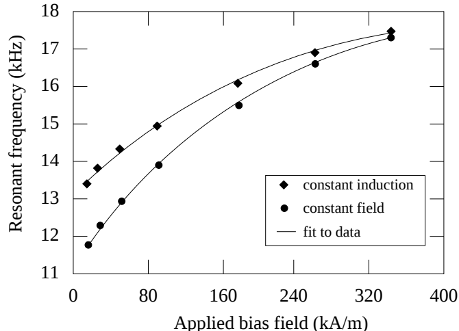
Figure 1: Resonant frequency at constant magnetic induction ( E^B ) and constant magnetic field ( E^H ) versus magnetic bias. (From [7]).
