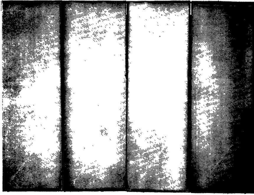
FIGURE 4.4: FIVE YEAR EXTERIOR TEST FENCE RESULTS (45° SOUTH IN A MARINE ENVIRONMENT) OF INORGANIC ZINC APPLIED TO FOUR DIFFERENT BLAST MEDIA PREPARED SURFACES
