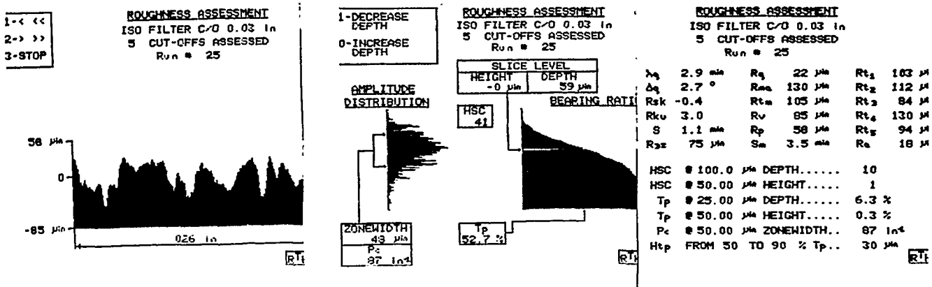
FIGURE 3.2: SAMPLE READOUT OF STYLUS INSTRUMENT
