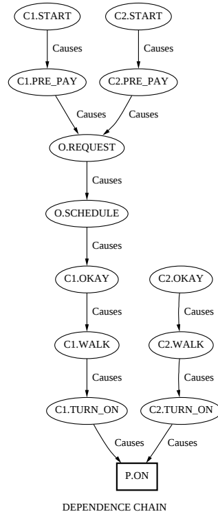
Figure 10: Aladdin-Generated Affected-By Chain.
