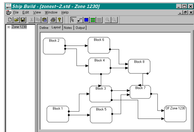
Figure 2. Ship Blocks Layout
